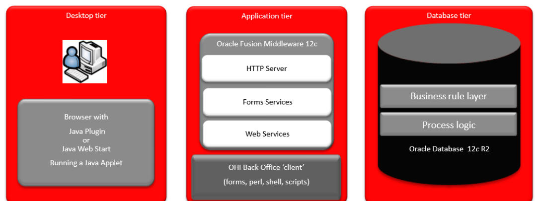
Figure 2: OHI Back Office GUI components
