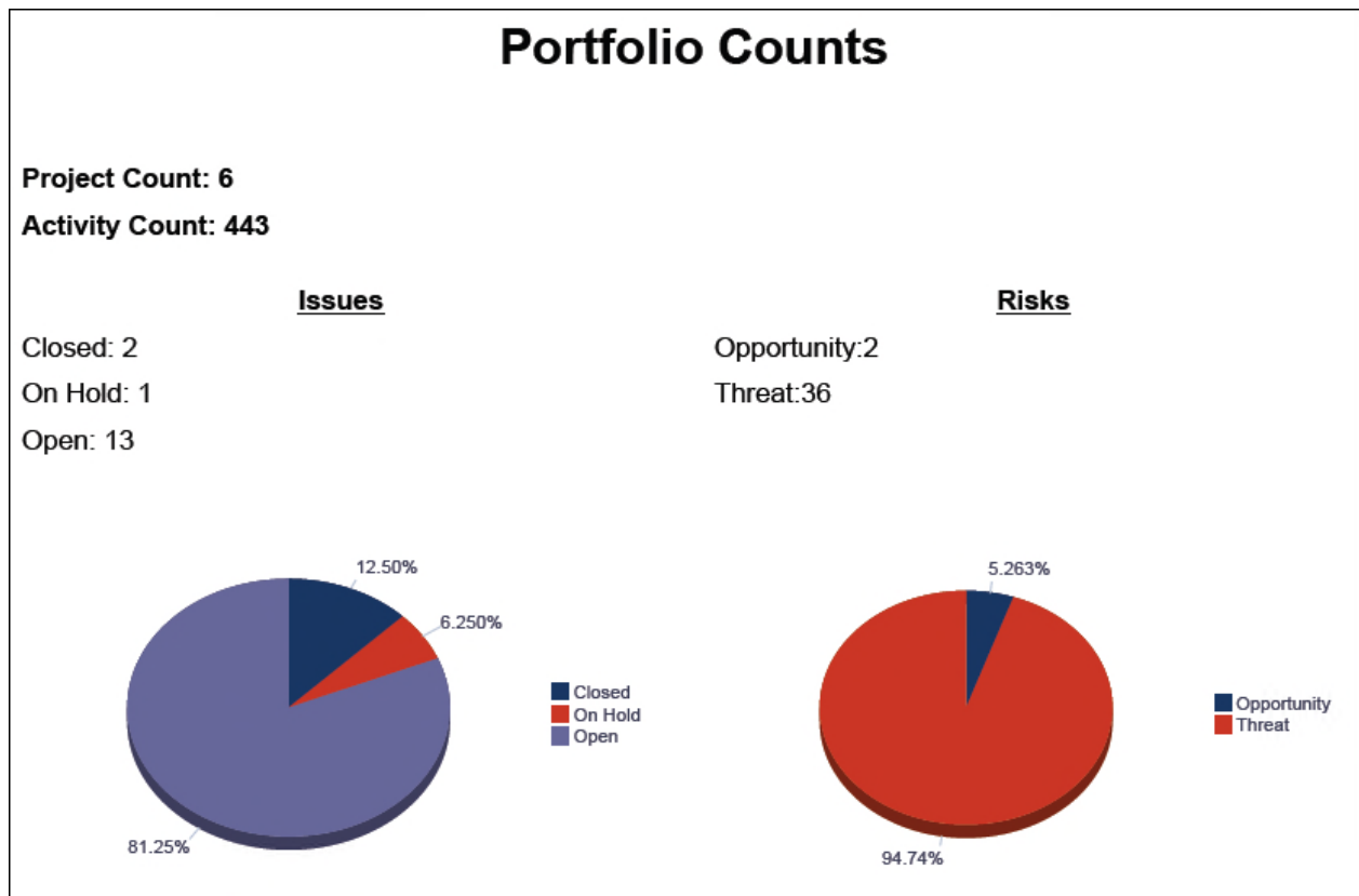
Figure 24: Portfolio Counts
