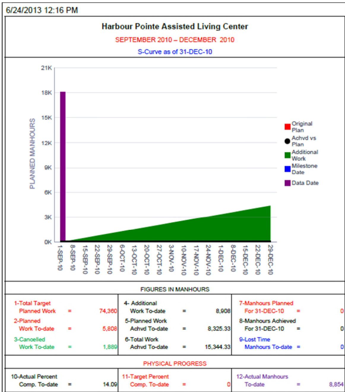
Figure 38: S Curve
