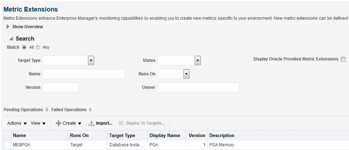
Figure 38-1 PGA Memory
