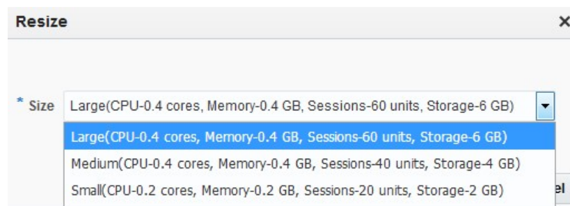
Figure 22-2 Resize Options
