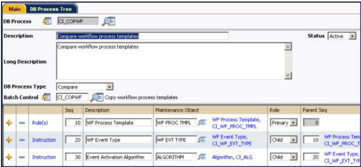
Figure 3: DB Process To Copy Workflow Process Templates
