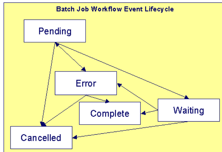
Figure 2: Workflow Event Lifecycle
