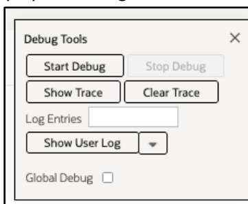
Figure 7: Debug Toolbar
