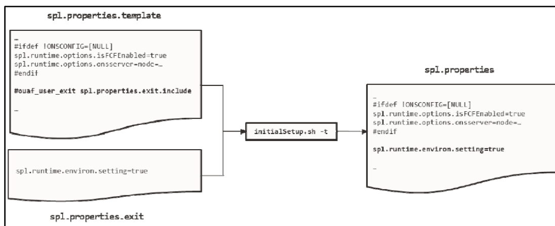
Figure 36: Include Files
