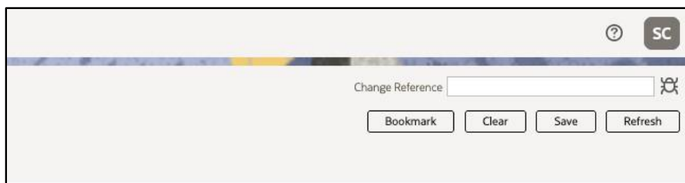
Figure 6: Debug Toolbar
