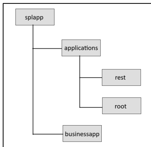
Figure 35: Expanded Format
