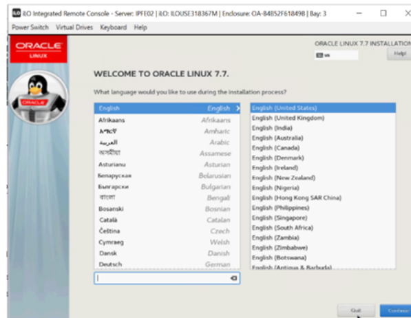
Figure 2-56 Language Selection
