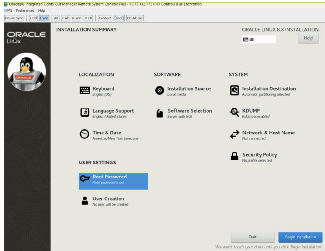
Figure 2-40 Root password
