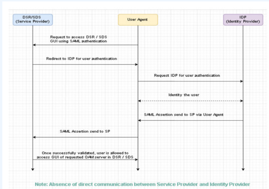
Figure 2-70 SAML Call Flow
