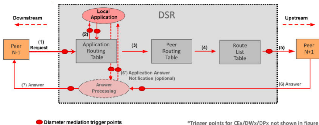
Figure 2-44 Mediation Trigger Points
