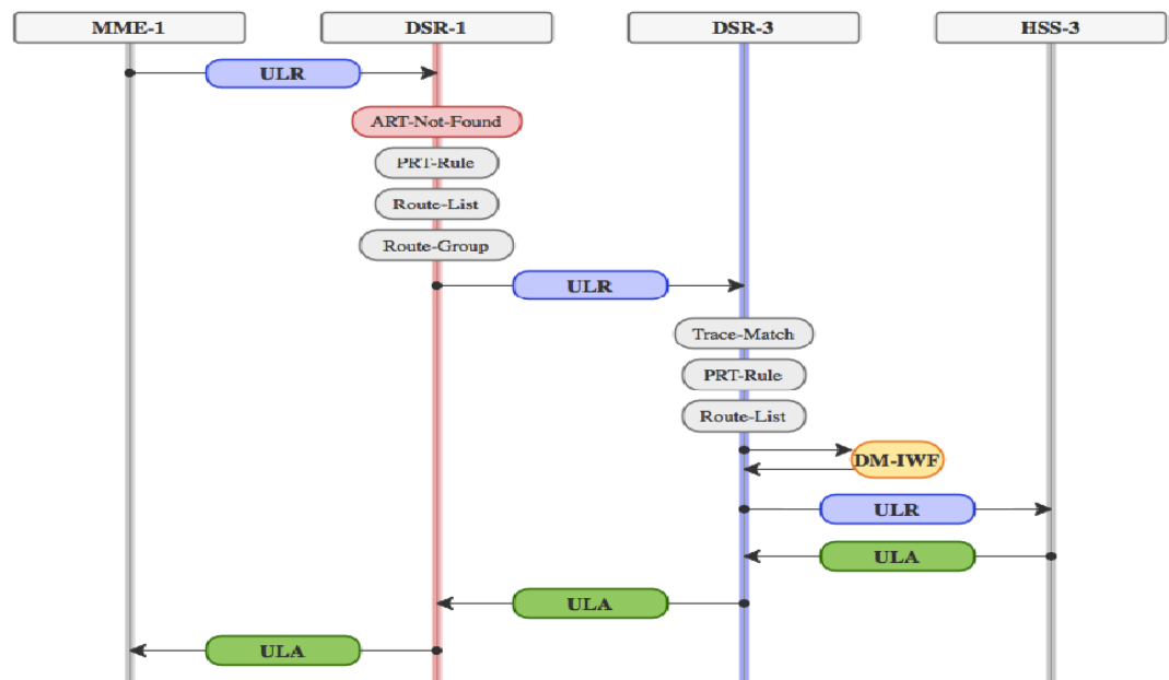
Figure 2-69 Message Flow for Network Wide Trace
