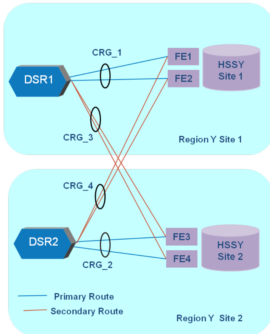
Figure 2-7 Connection Route Group
