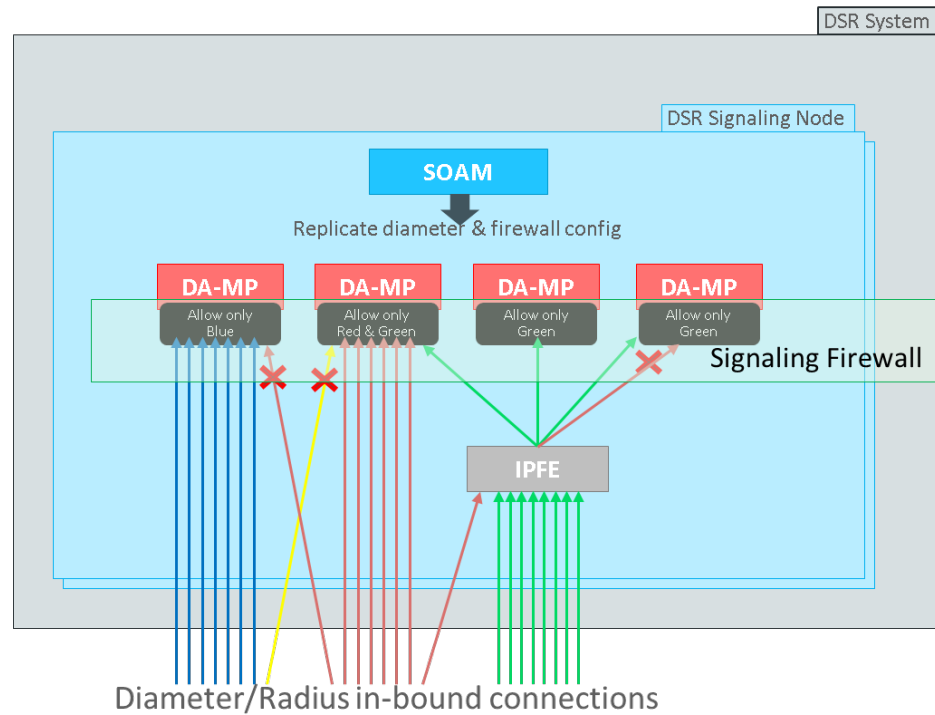
Figure 2-15 DSR Signaling Firewall
