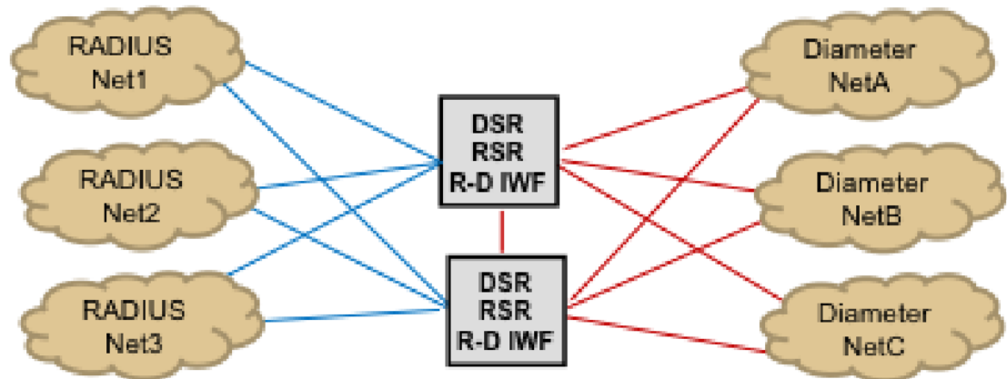
Figure 2-42 RSR and R-D IWF Deployment
