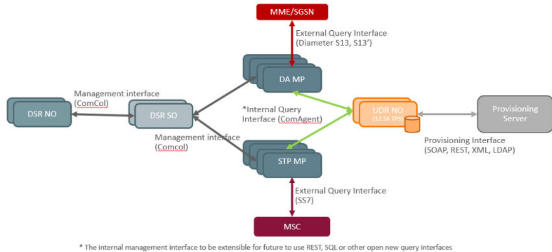
Figure 2-73 EIR solution architecture.
