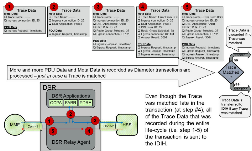
Figure 2-67 IDIH Trace Data
