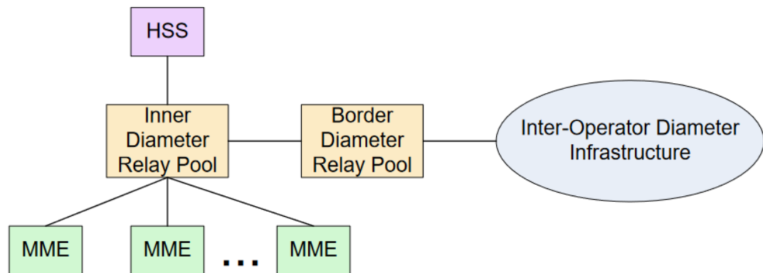
Figure 1-2 3GPP Inter/Intra-operator Diameter infrastructure
