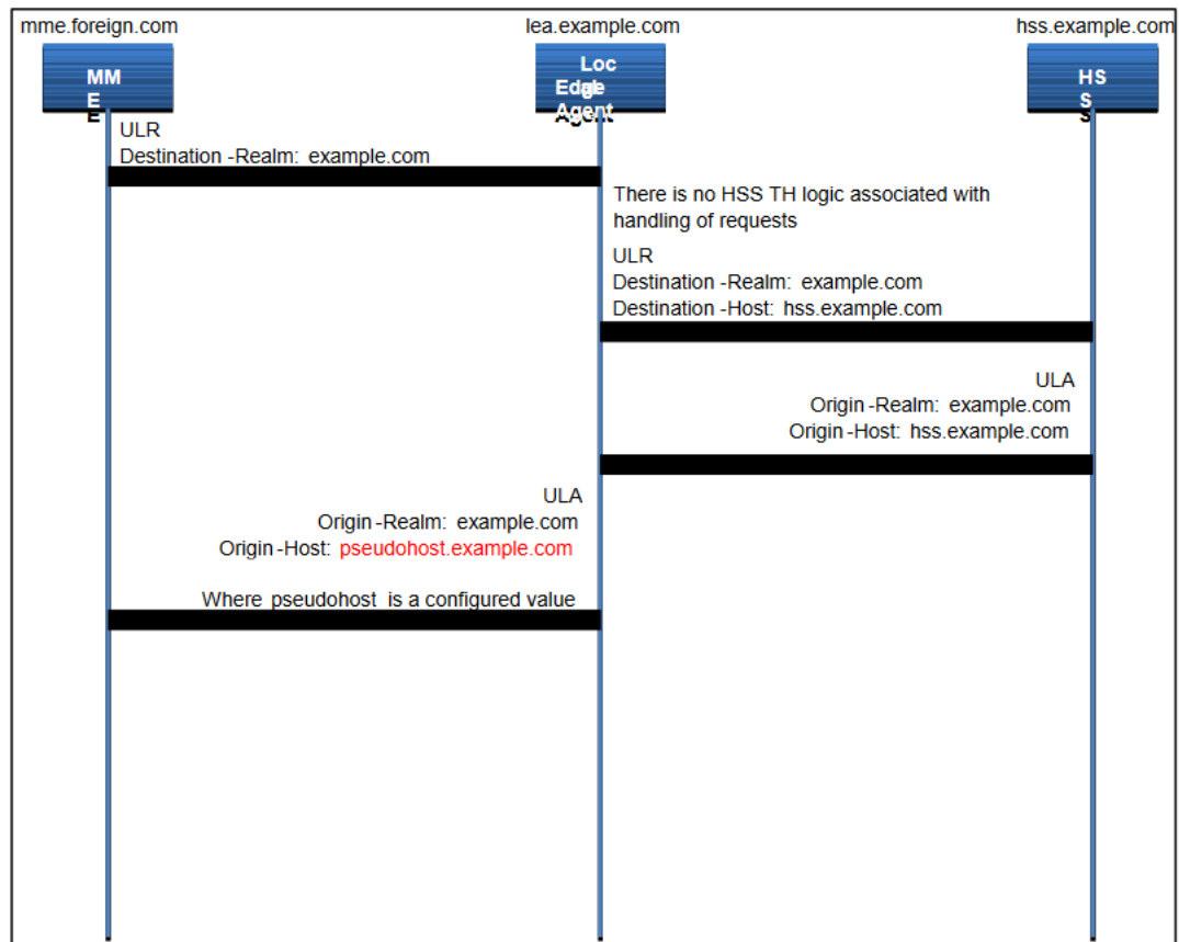
Figure 2-46 S6a/S6d HSS Topology Hiding - ULR Message Flow
