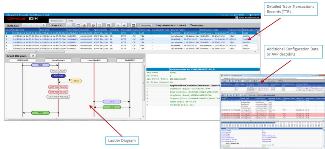
Figure 2-68 IDIH Visualization GUI
