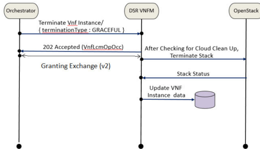
Figure 15-2 Graceful termination
