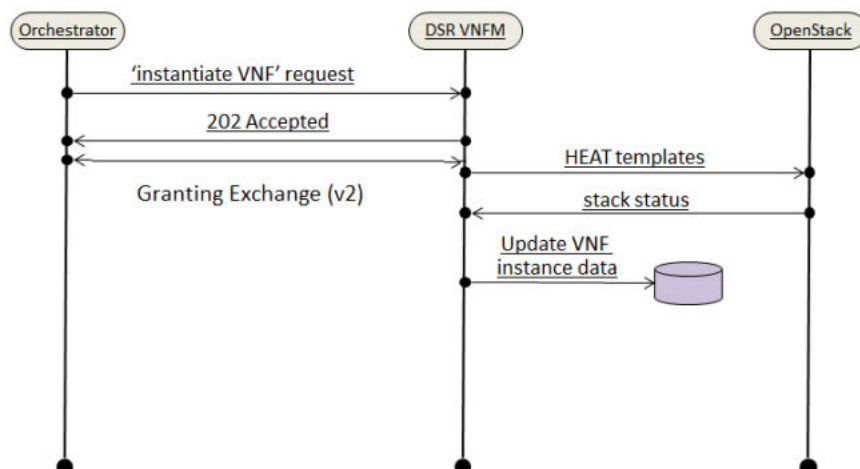
Figure 10-5 VNF installation
