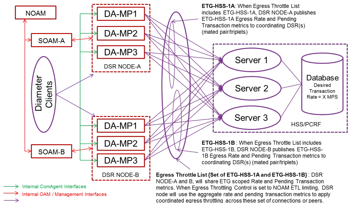
Figure 2-23 2 DSR Sites- Coordinated Egress Throttling Example
