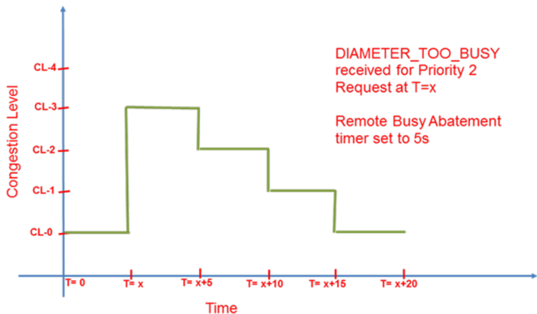
Figure 2-25 Congestion level abatement over time for Remote Busy
