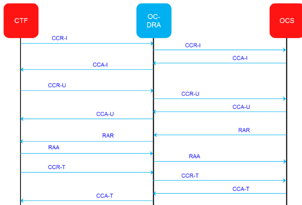
Figure 2-52 A typical Online Charging Session
