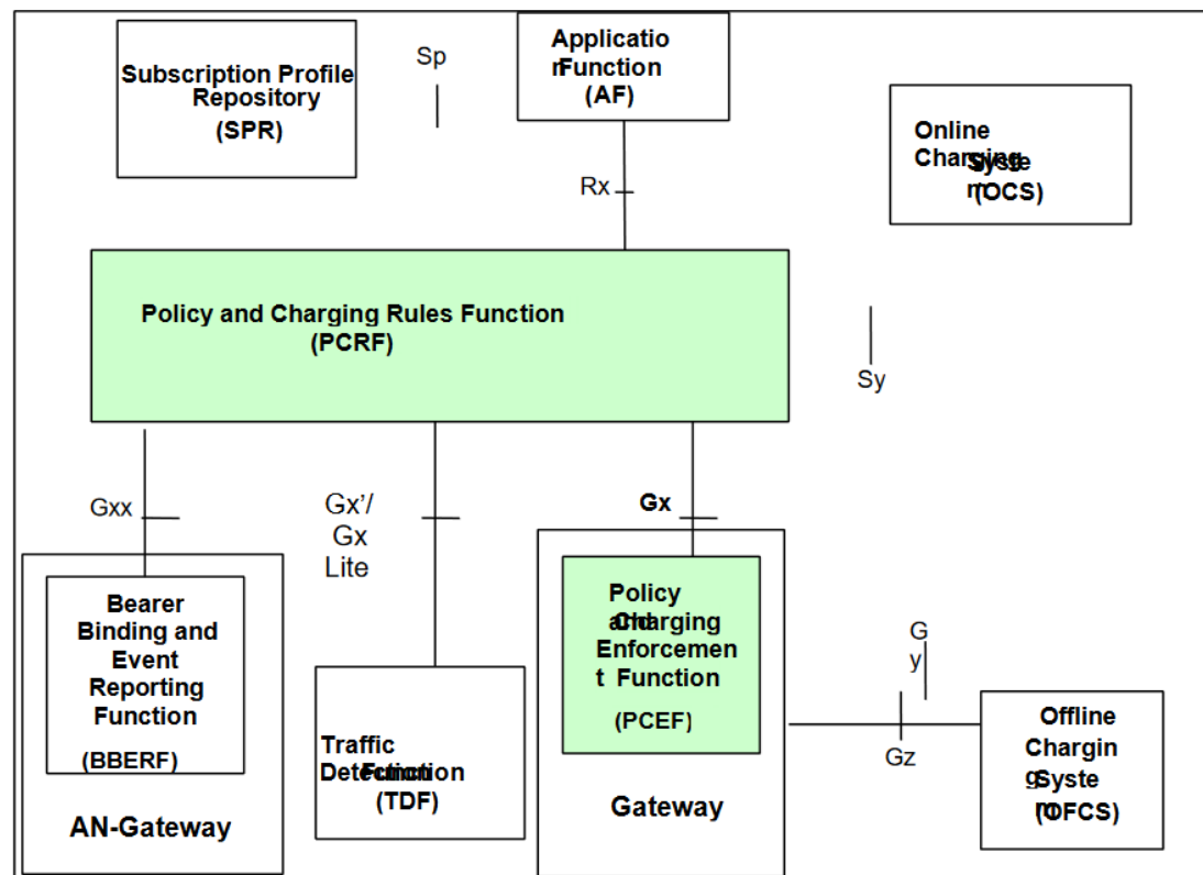
Figure 2-54 Overall PCC logical architecture (non-roam)
