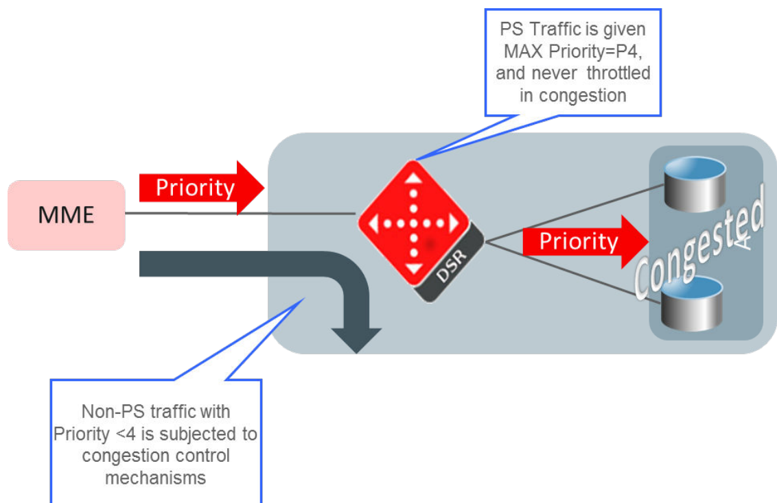
Figure 2-37 NGN-PS Support
