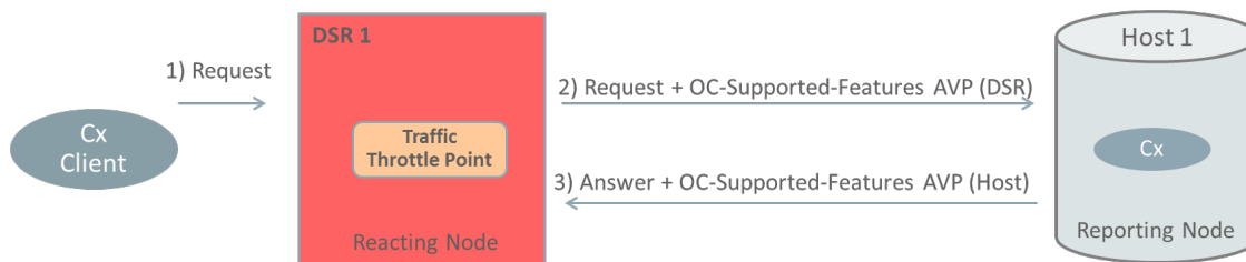
Figure 2-27 DOIC Capabilities Announcement
