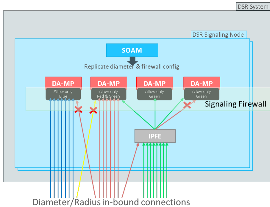
Figure 2-15 DSR Signaling Firewall
