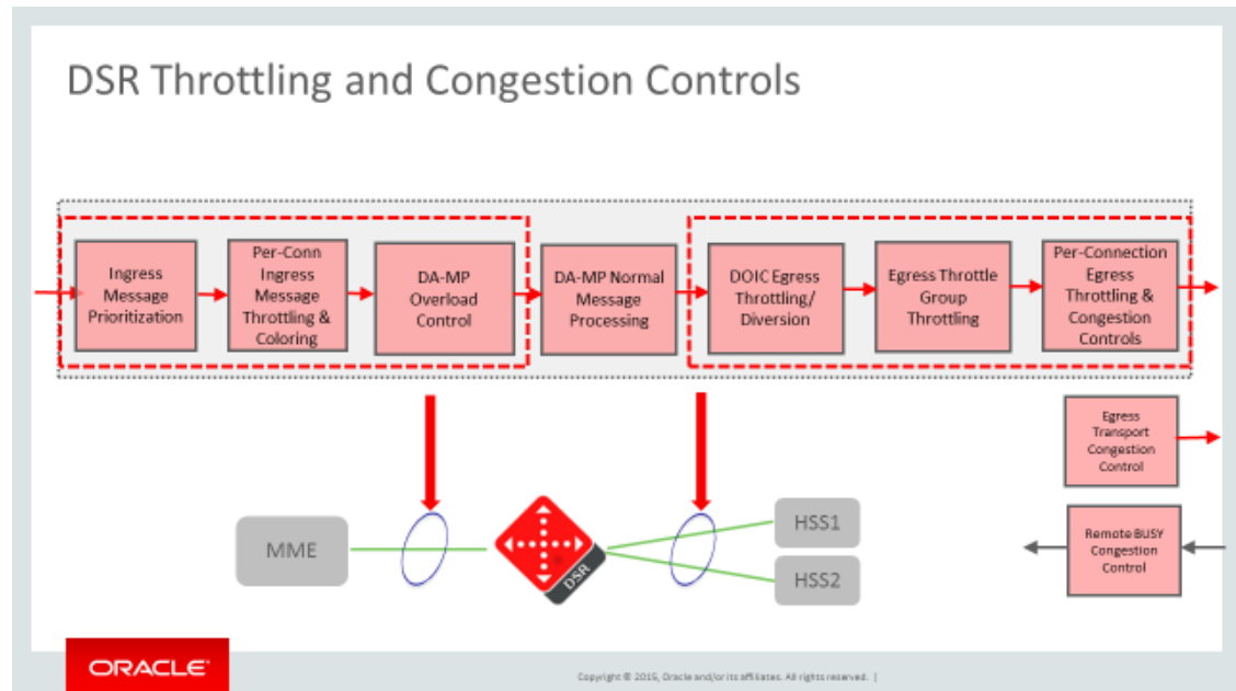
Figure 2-17 Congestion Control
