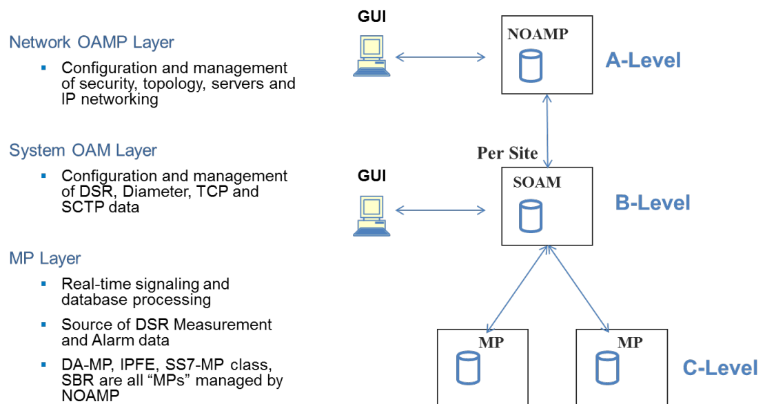
Figure 2-2 DSR 3-tiered Topology Architecture
