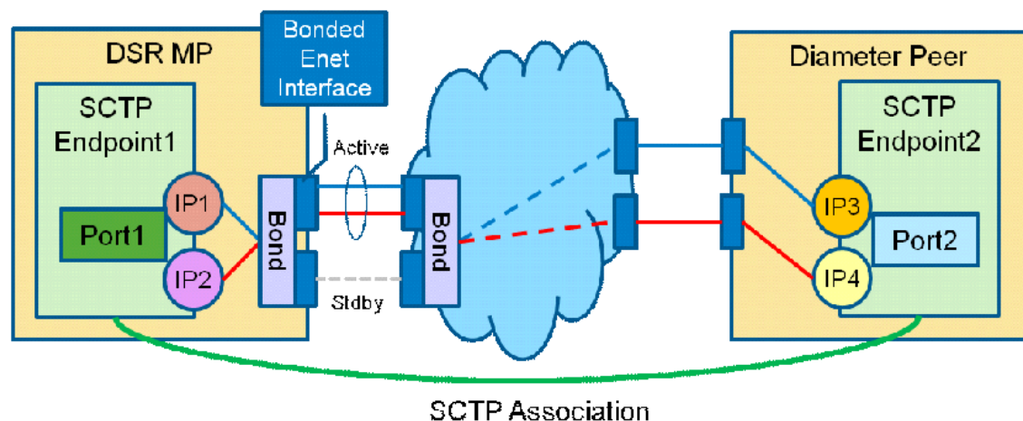
Figure 2-12 SCTP Multi-Homing via Port Bonding
