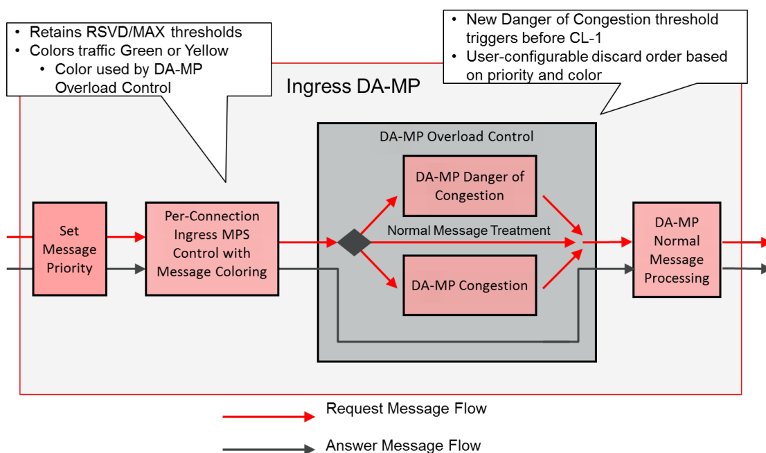
Figure 2-19 Message Coloring and Priority or Color based DA-MP Overload Control
