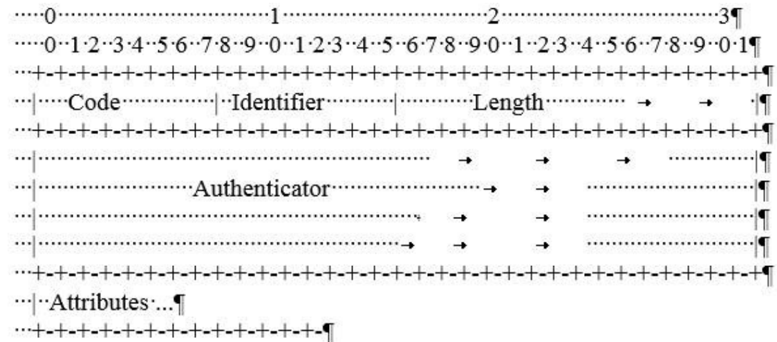
Figure 2-40 RADIUS Data Format
