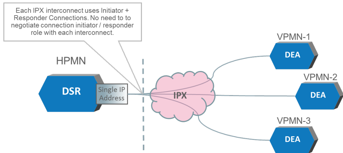
Figure 2-38 IPFE Initiator or Responder Support
