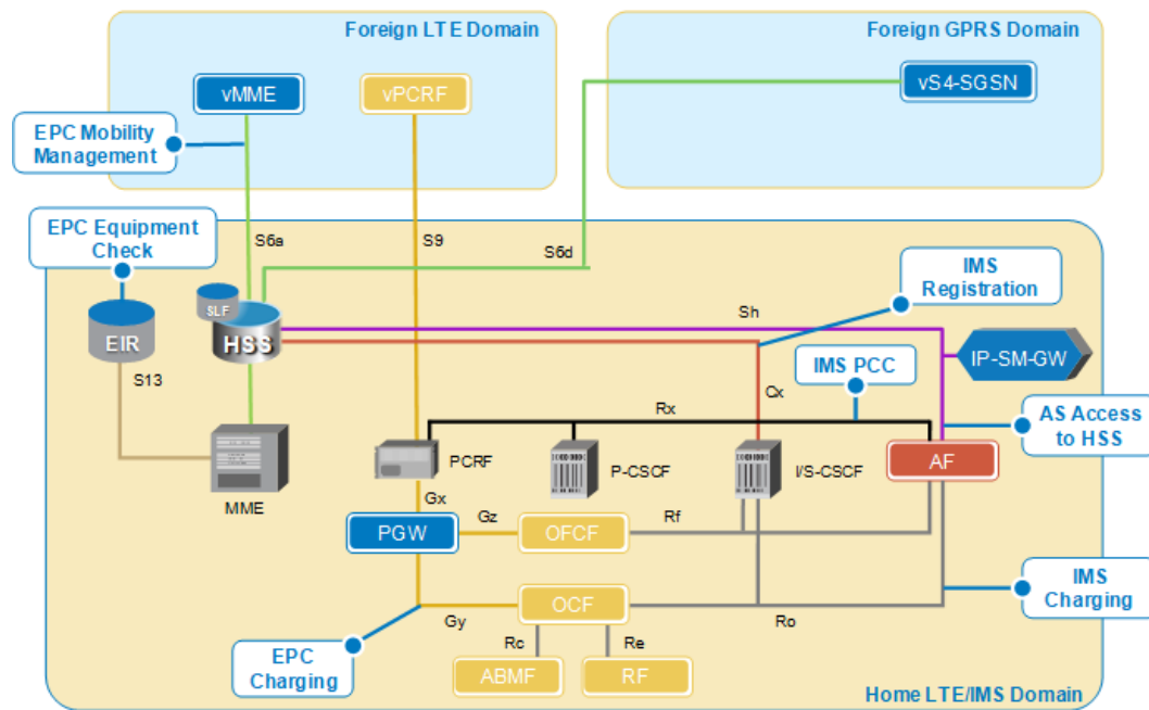
Figure 1-1 Selected Diameter Interfaces in LTE and IMS
