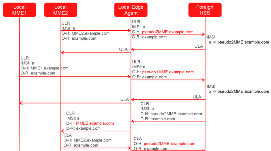
Figure 2-45 MME/SGSN Topology Hiding
