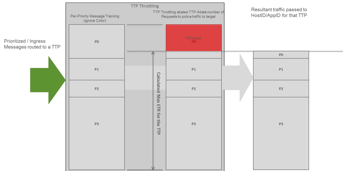
Figure 2-30 Throttle by Message Priority Only when support for 5 message priorities is enabled
