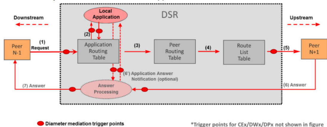
Figure 2-44 Mediation Trigger Points
