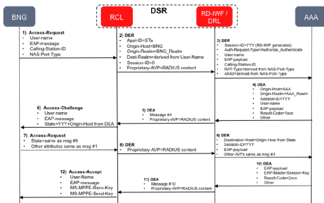
Figure 2-43 RADIUS-Diameter IWF for Authentication
