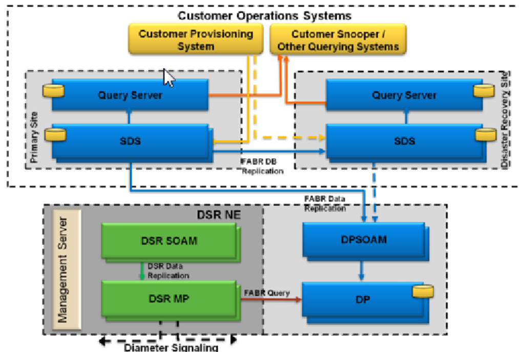
Figure 2-49 Subscriber Data Server Architecture
