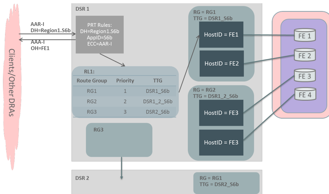
Figure 2-34 Congestion-Aware Route List Example 1
