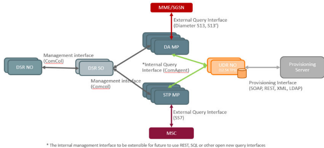
Figure 2-71 EIR solution architecture.
