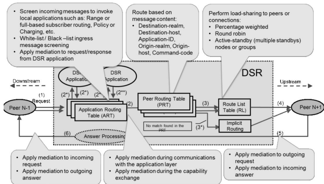
Figure 2-6 High Level Message Processing and Routing in DSR
