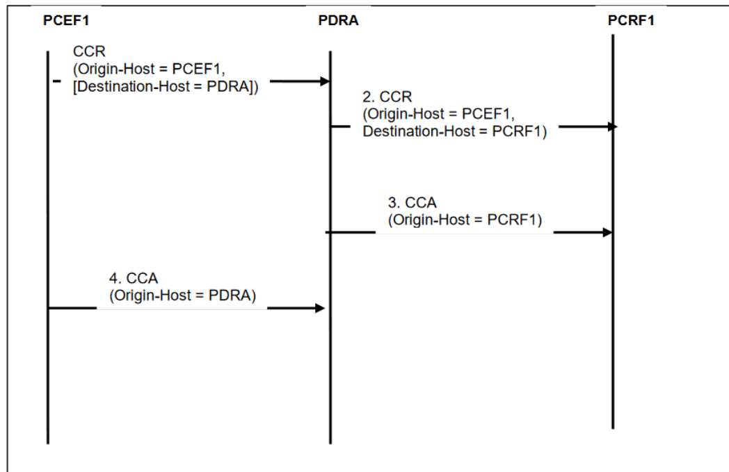
Figure 2-55 PCRF topology hiding
