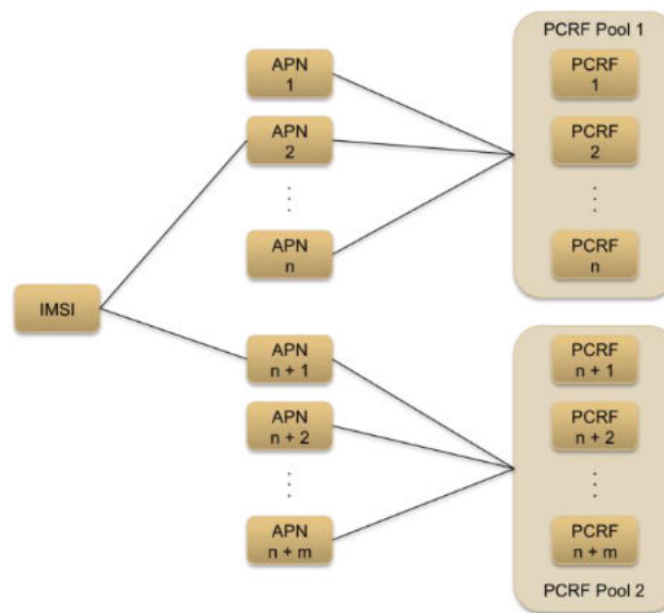
Figure 2-57 Relationship between IMSIs and PCRF pools
