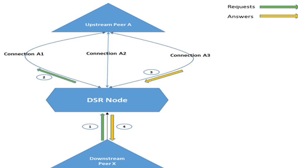
Figure 2-16 Answer processing on connection different from the connection used to send Request message
