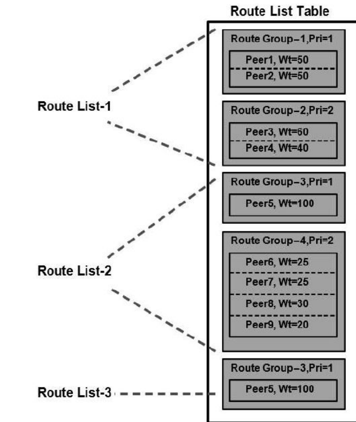
Figure 2-8 Route List, Route Group, Peer Relationship Example
