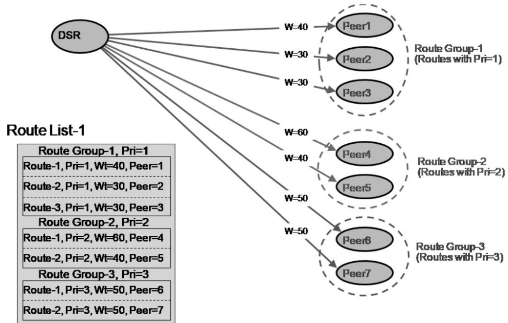
Figure 2-9 Load Balancing Based on Route Groups and Peer Weights
