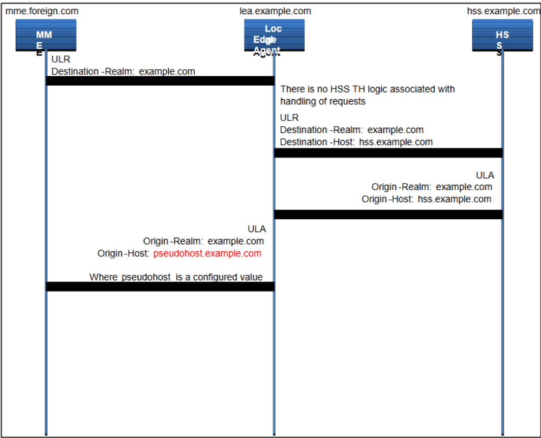
Figure 2-46 S6a/S6d HSS Topology Hiding - ULR Message Flow
