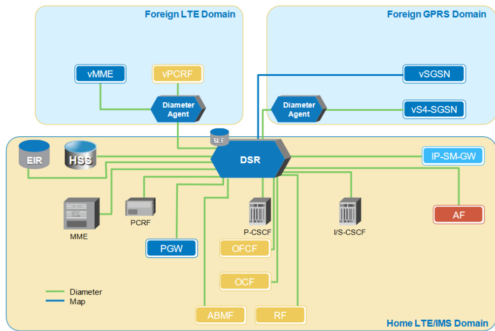
Figure 1-4 Example of Operator's EPC/IMS Core network with DSR
