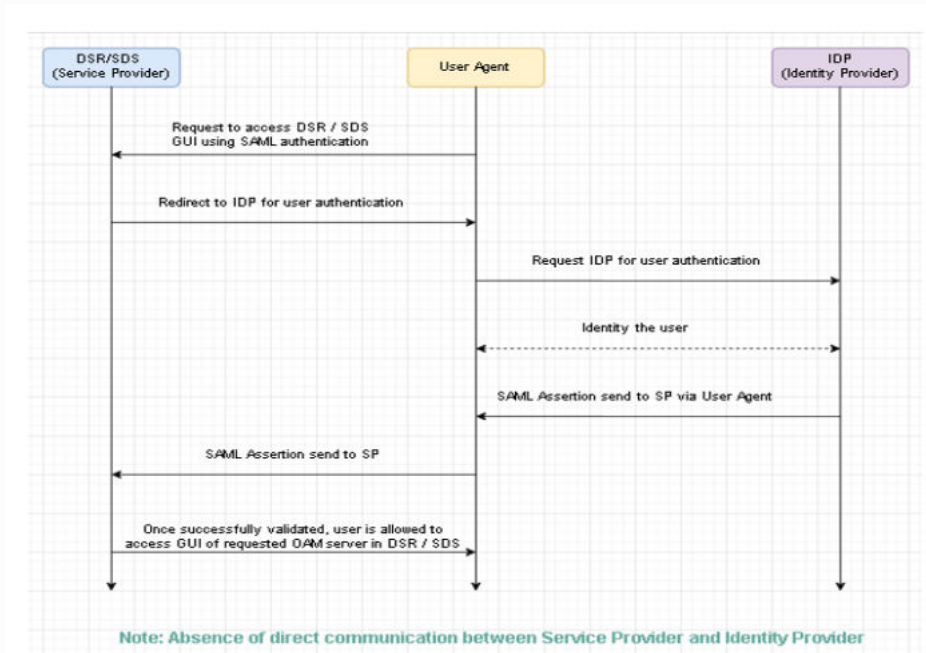
Figure 2-67 SAML Call Flow
