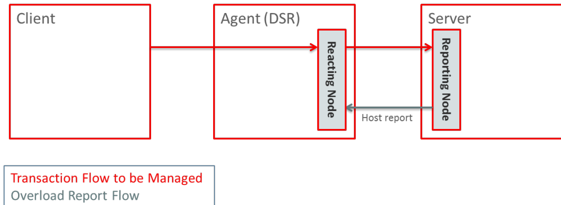
Figure 2-26 Reacting Node Role for DOIC
