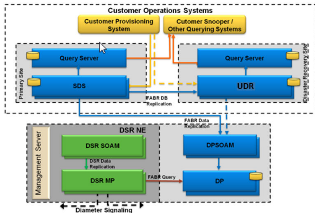
Figure 2-50 User Data Repository Architecture
