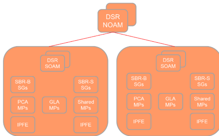
Figure 2-60 PCA and GLA NOAM Architecture
