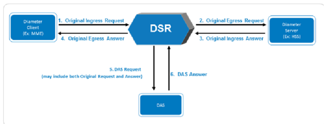
Figure 2-63 Message Copy Overview
