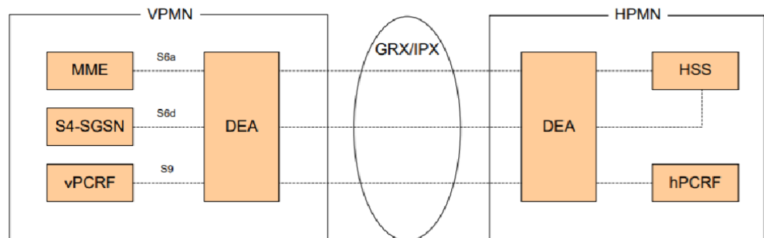
Figure 1-3 GSMA roaming implementation architecture
