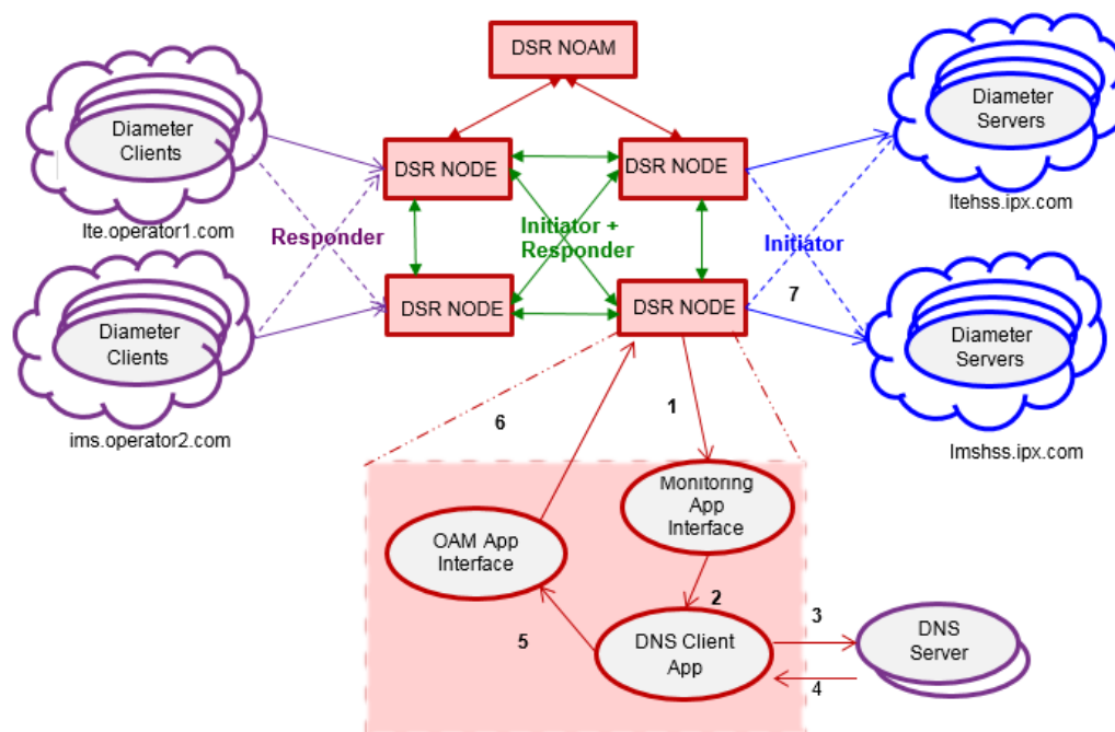
Figure 2-13 Dynamic Diameter Peer Discovery: Example
