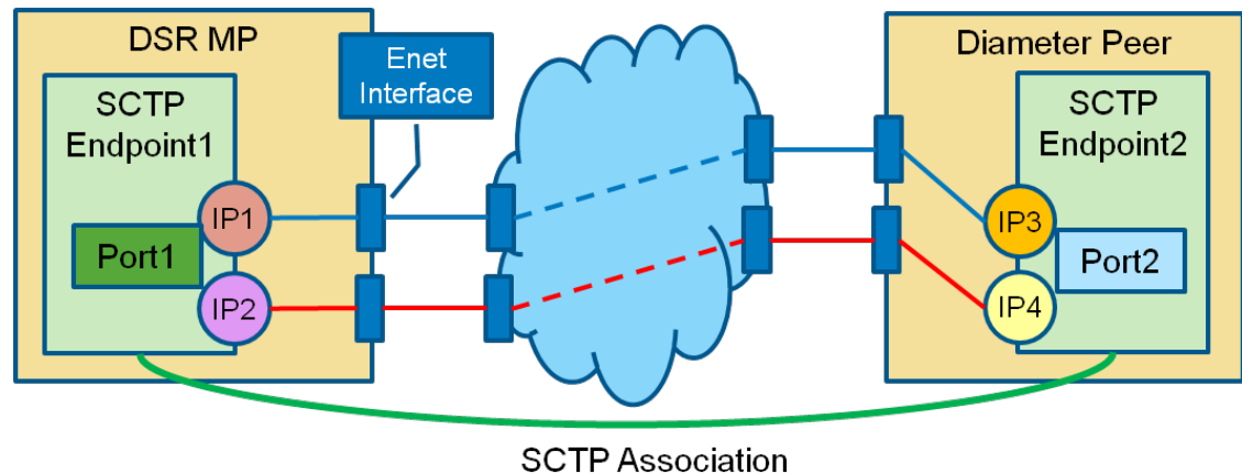
Figure 2-11 SCTP Multi-Homing
