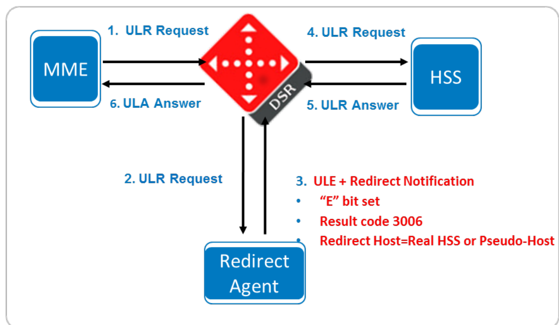
Figure 2-10 Redirect Agent
