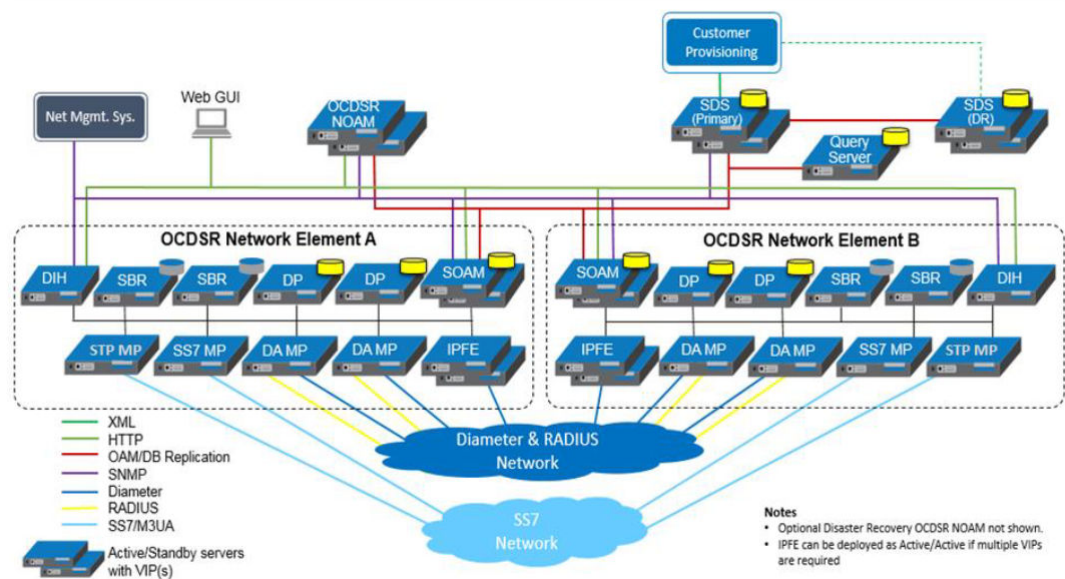
Figure 2-1 DSR 7.x Architecture
