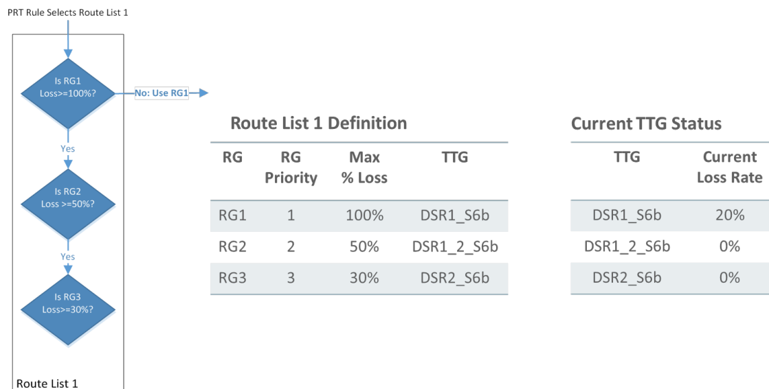
Figure 2-33 Congestion-Aware Route List Logic
