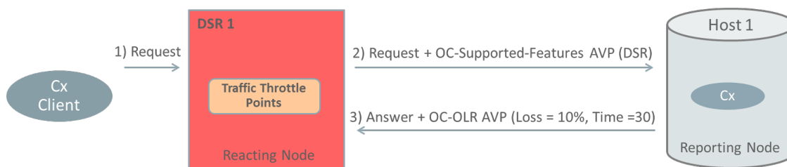
Figure 2-28 DOIC Overload Reports Example
