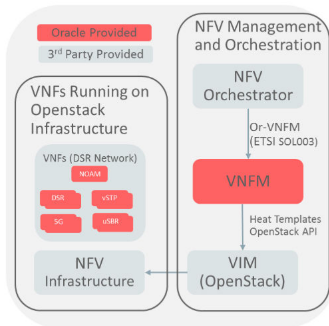
Figure 2-64 DSR VNFM
