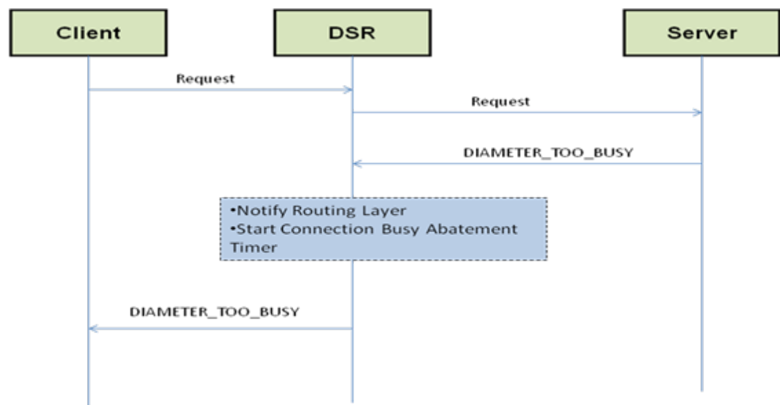
Figure 2-24 Connection Busy
