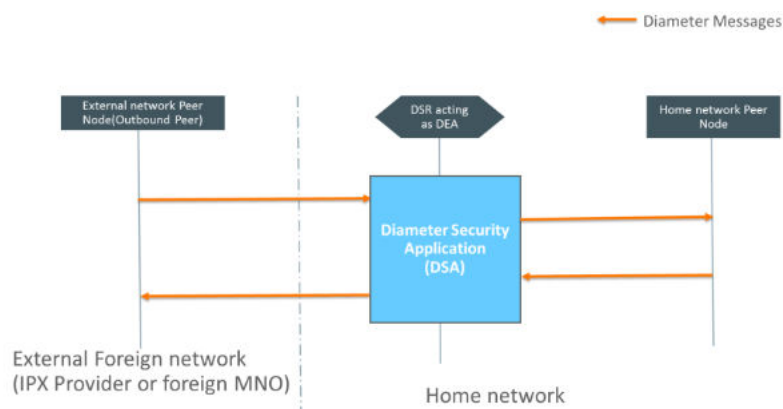
Figure 2-62 Diameter Security Application (DSA)
