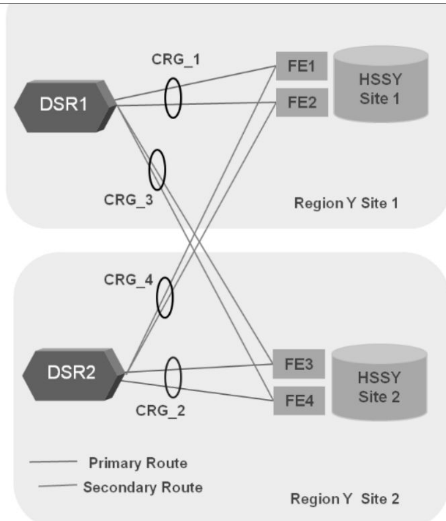
Figure 2-7 Connection Route Group
