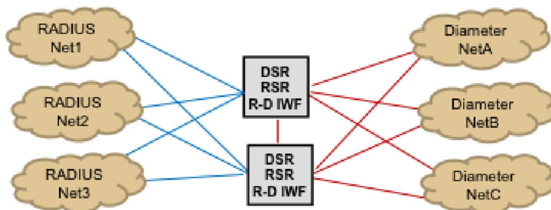
Figure 2-42 RSR and R-D IWF Deployment
