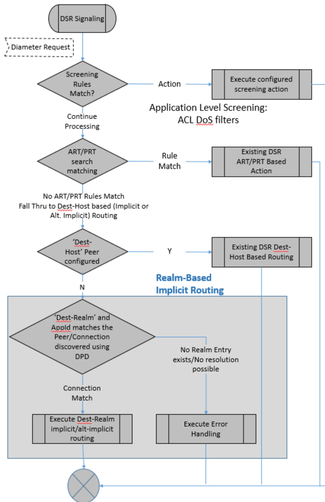
Figure 2-14 High Level DSR Routing Flow – Fall through to Dest-Realm Based Implicit Routing
