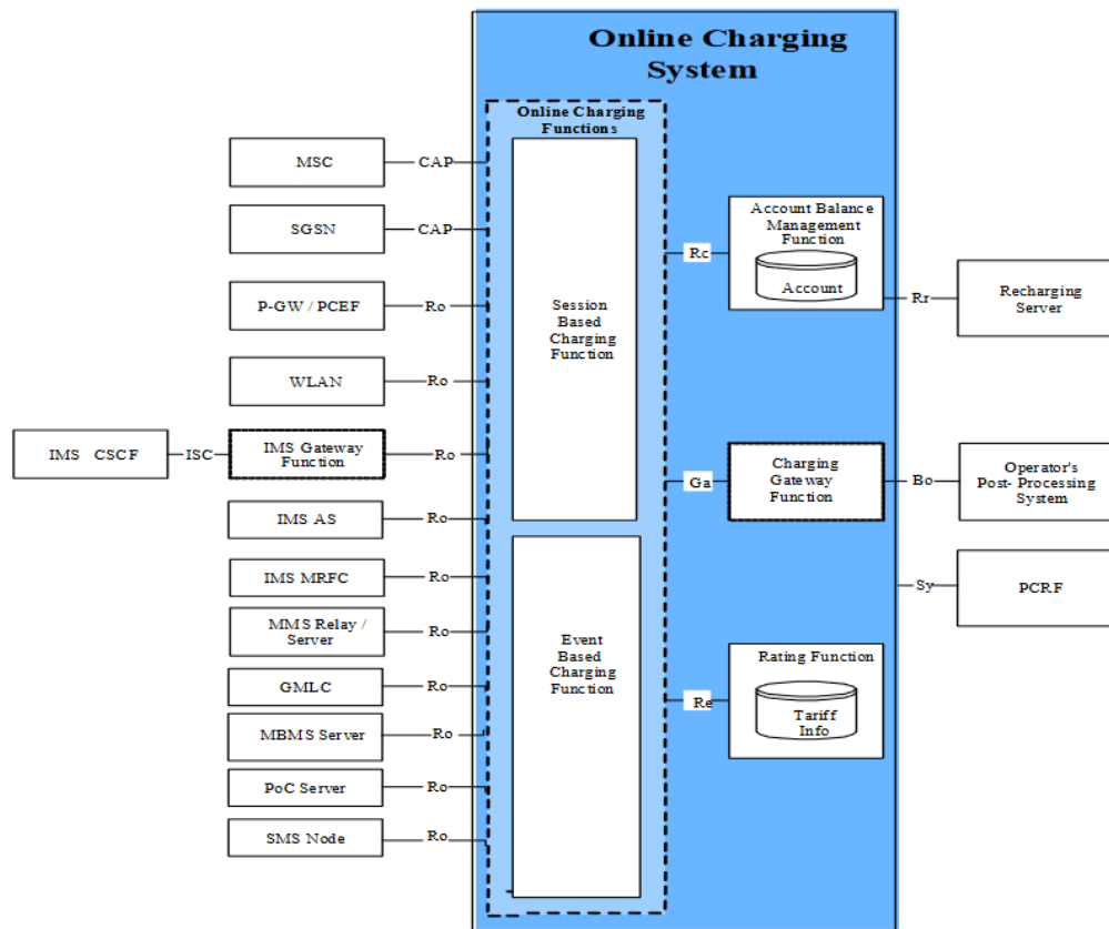
Figure 2-51 Online Charging System and Architecture
