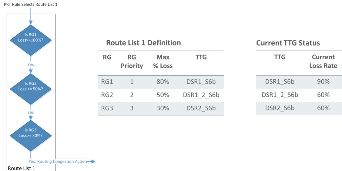
Figure 2-36 Congestion-Aware Route List Logic Example 1b
