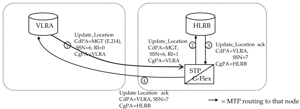
Figure 6-1 E.214 (E.212) Routing Example - Location Updating
