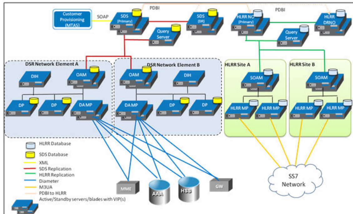
Figure 2-2 SDS/HLRR Architecture Overview
