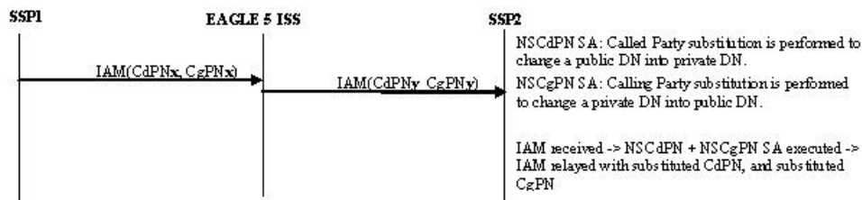
Figure 2-11 ISUP RELAY with TIF NS
