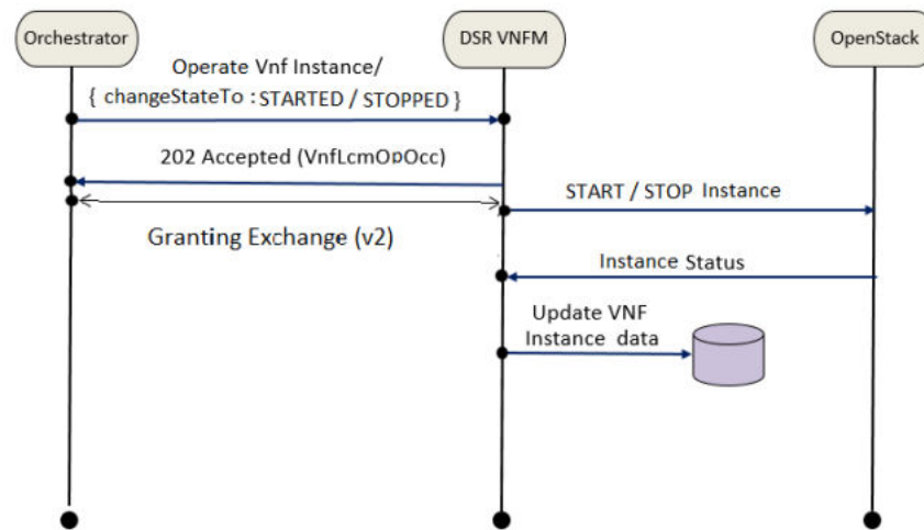
Figure 10-8 Operate vnf
