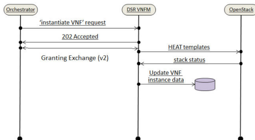
Figure 10-5 VNF installation
