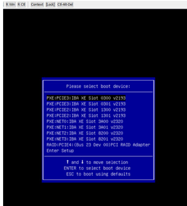
Figure A-3 ILOM Boot process
