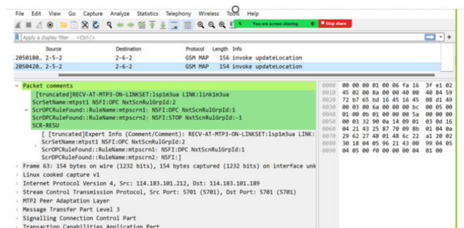
Figure 2-34 MTP3 Screened Message
