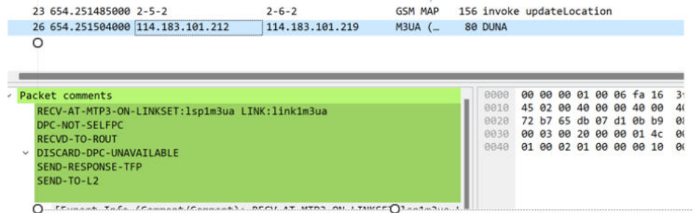
Figure 2-35 MTP3 Routed Message
