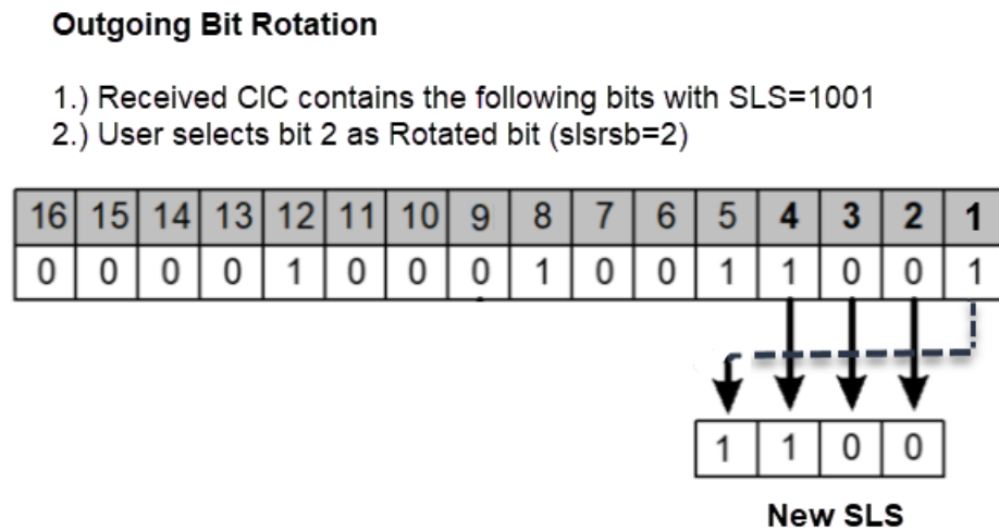
Figure 2-10 Example: SLS Outgoing Bit Rotation
