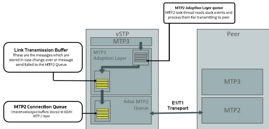
Figure 2-5 MTP2 Link Congestion Detection
