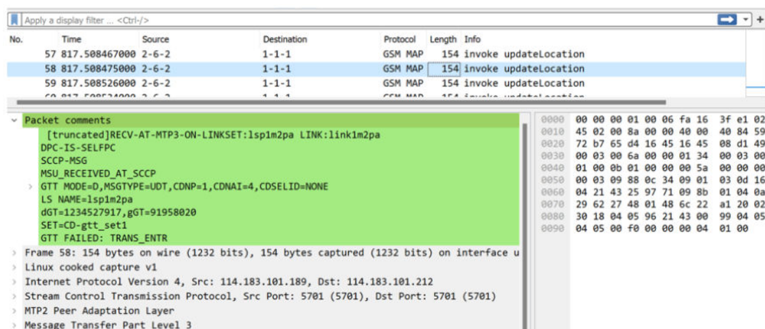
Figure 2-26 SCCP Routed Message
