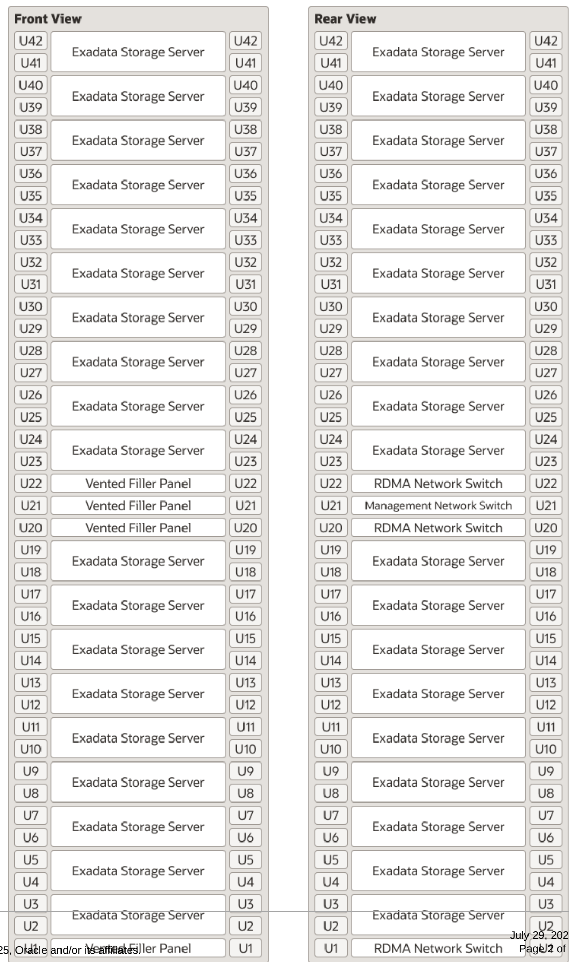
Figure 22-1 Rack Layout for Oracle Exadata Storage Expansion Rack X11M and X10M
