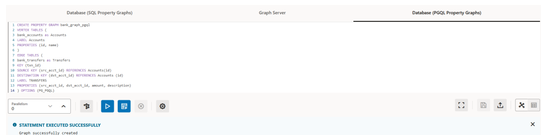
Figure 22-11 Creating a PGQL property graph
