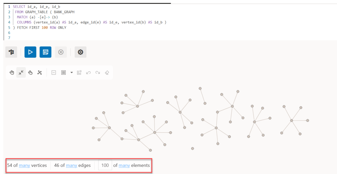
Figure 22-18 Default Display Size
