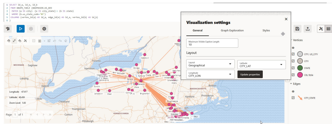
Figure 22-26 Geographical Layout
