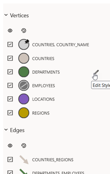
Figure 22-17 Graph Legends
