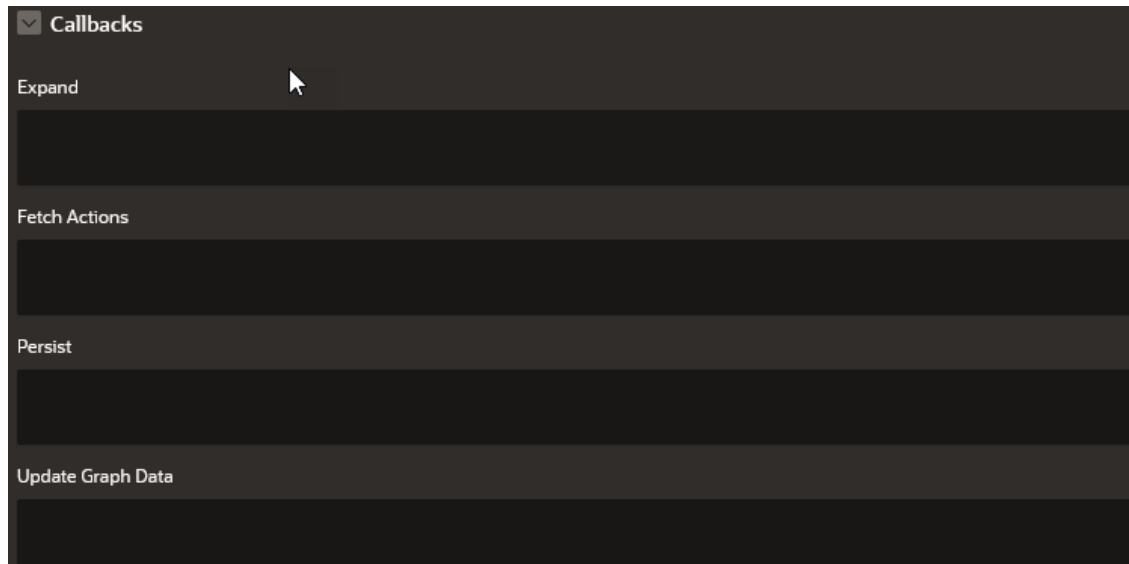
Figure 9-16 Callbacks
