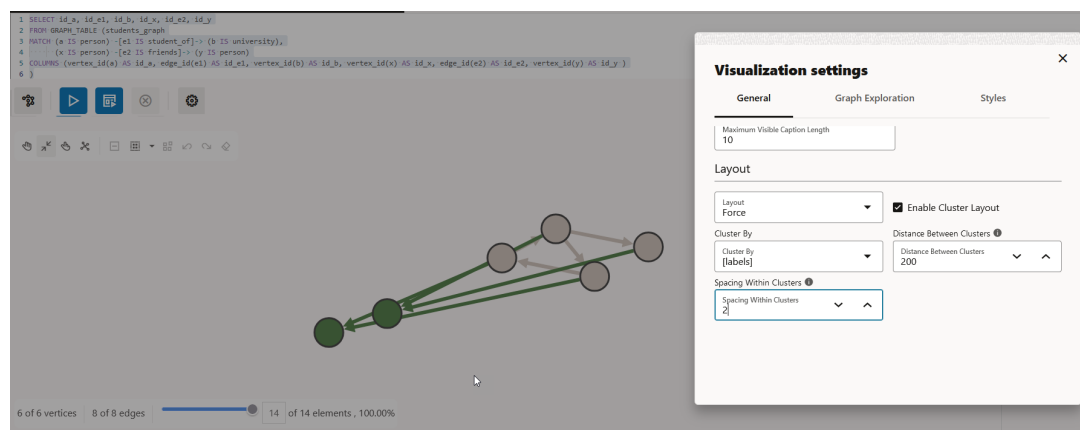
Figure 22-25 Cluster-Based Layout
