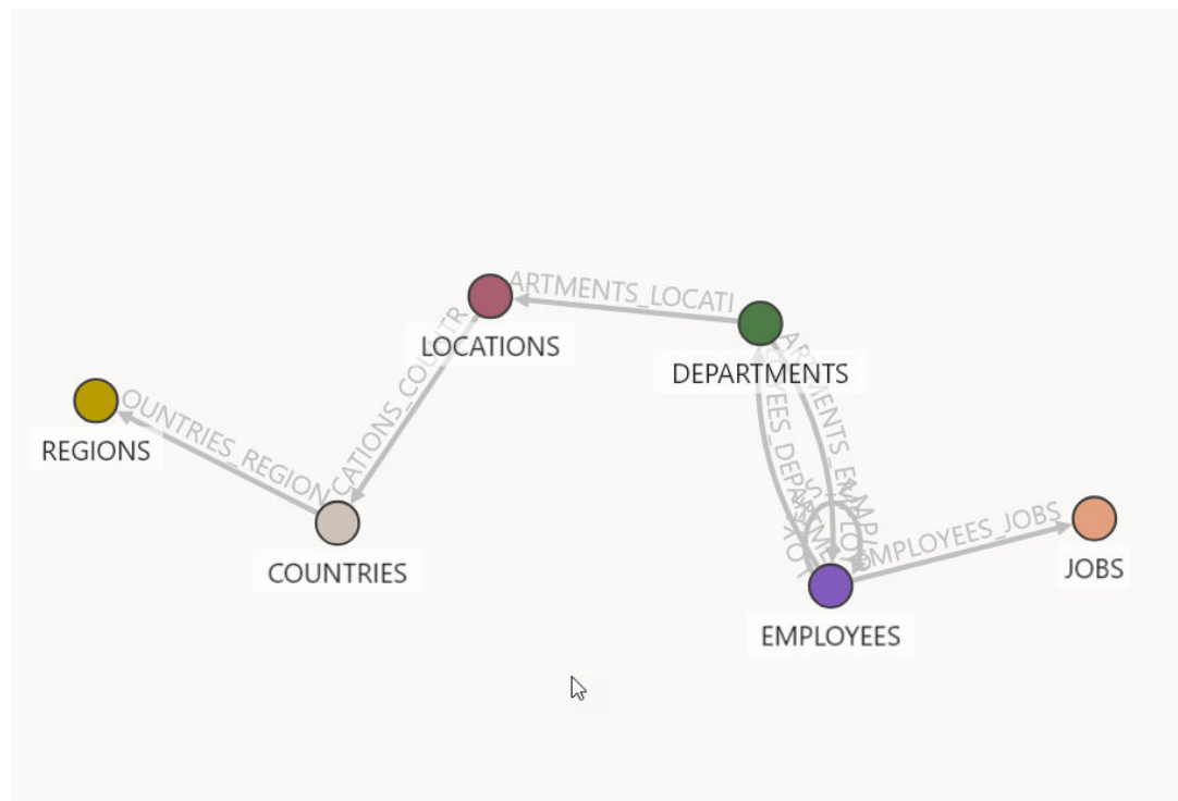
Figure 22-5 Graph Schema Visualization
