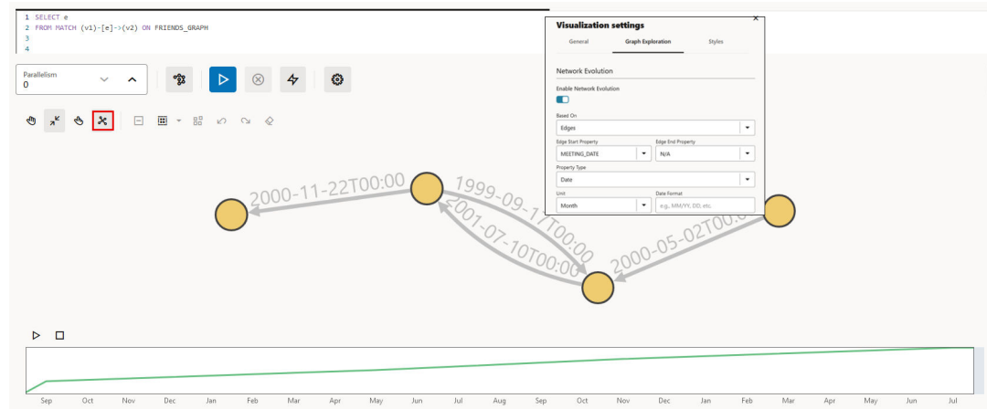
Figure 22-27 Dynamic Graph Visualization
