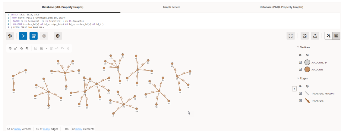
Figure 22-3 Graph Query on a SQL Property Graph
