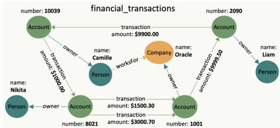
Figure 10-2 Financial Transactions Graph
