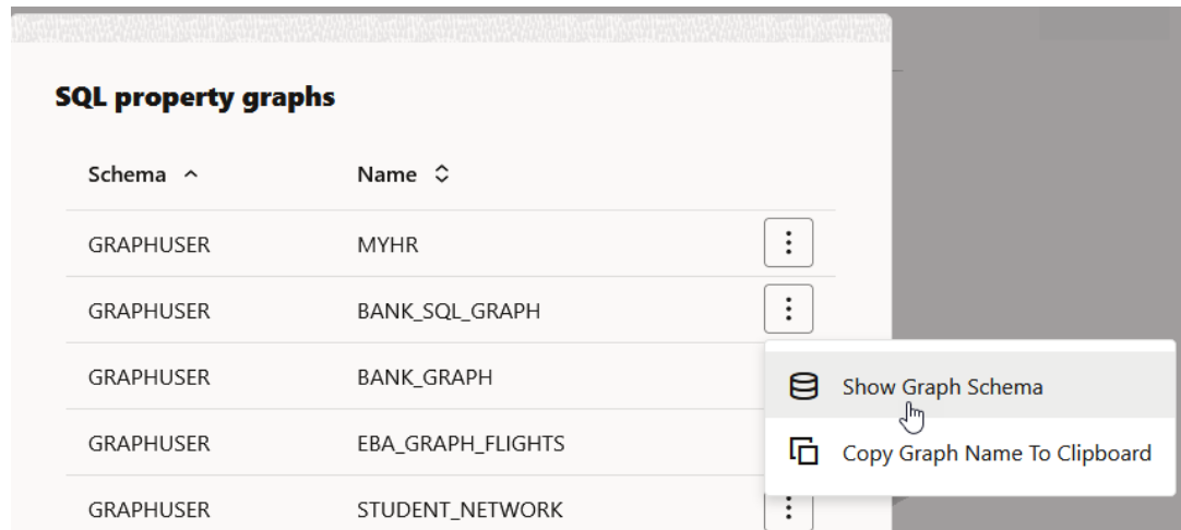
Figure 22-4 Show Graph Schema Option
