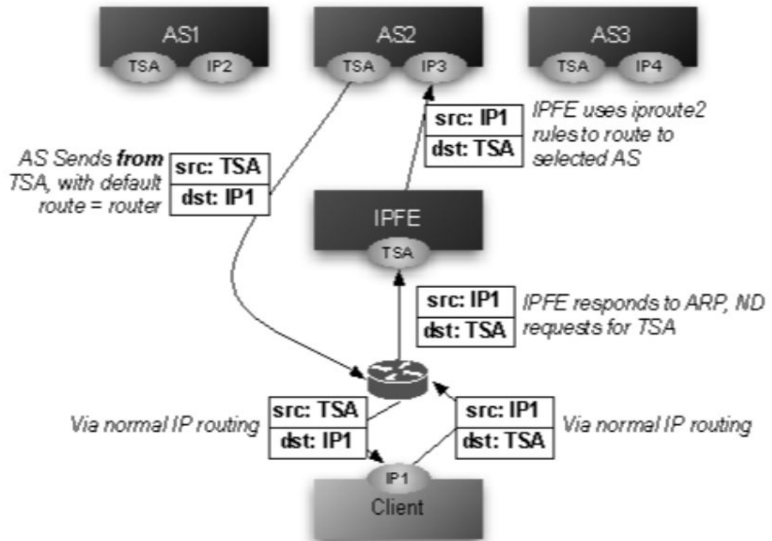
Figure 2-2 Packet Routing Through and Around the IPFE
