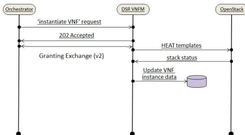
Figure 10-5 VNF installation
