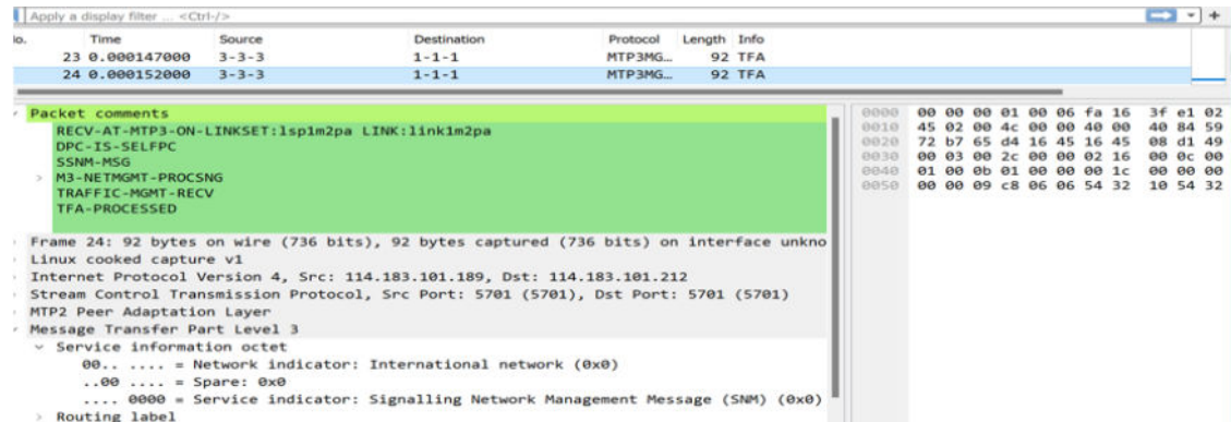
Figure 2-31 SNM - TFA
