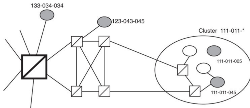
Figure 2-50 Cluster Routing
