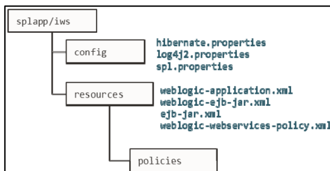
Figure 25: Inbound Web Services Configuration
