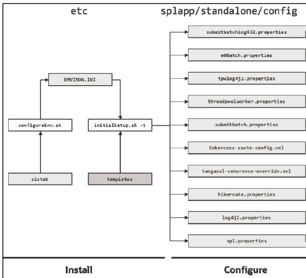
Figure 31: Batch Configuration Process
