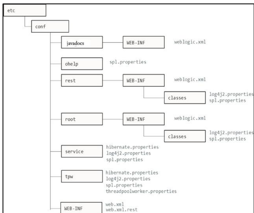
Figure 18: Configuration File Hierarchy
