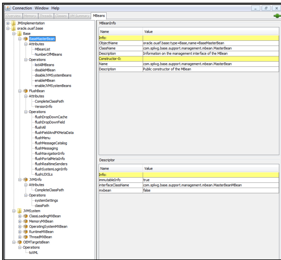
Figure 9: Example Web Application Server Mbeans in jconsole
