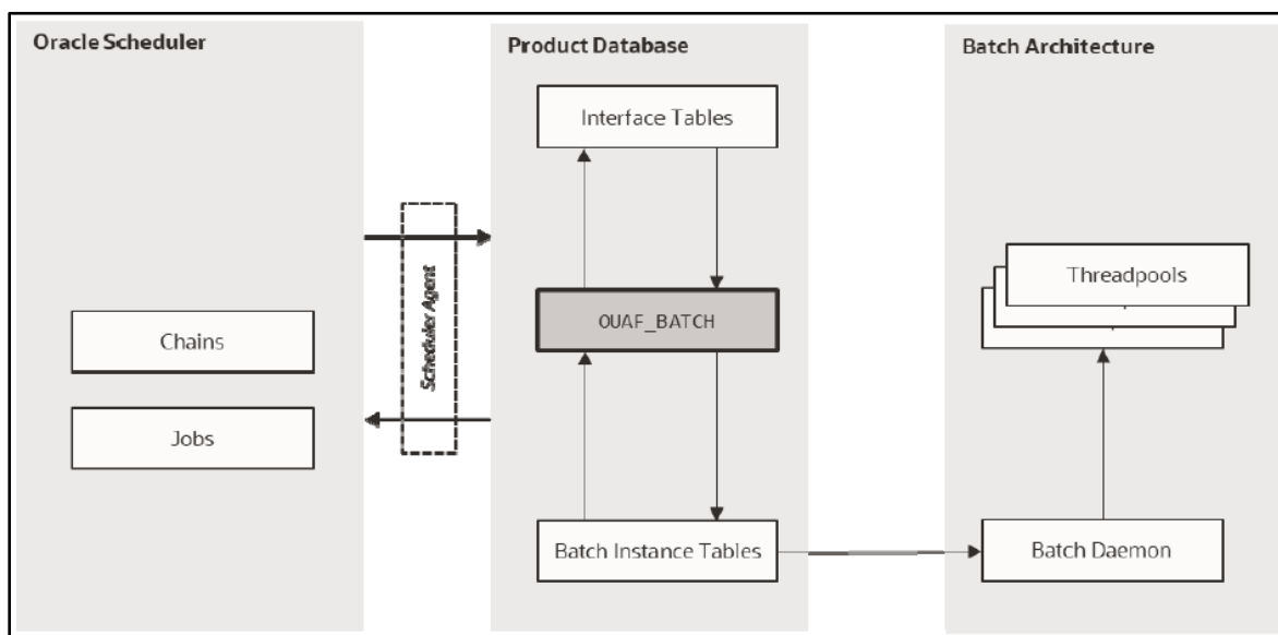
Figure 45: Oracle Scheduler Interface
