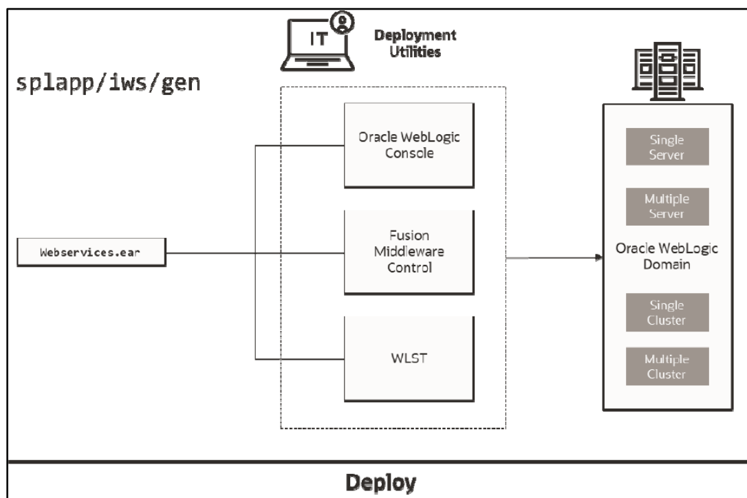
Figure 28: Inbound Web Services Deployment Process
