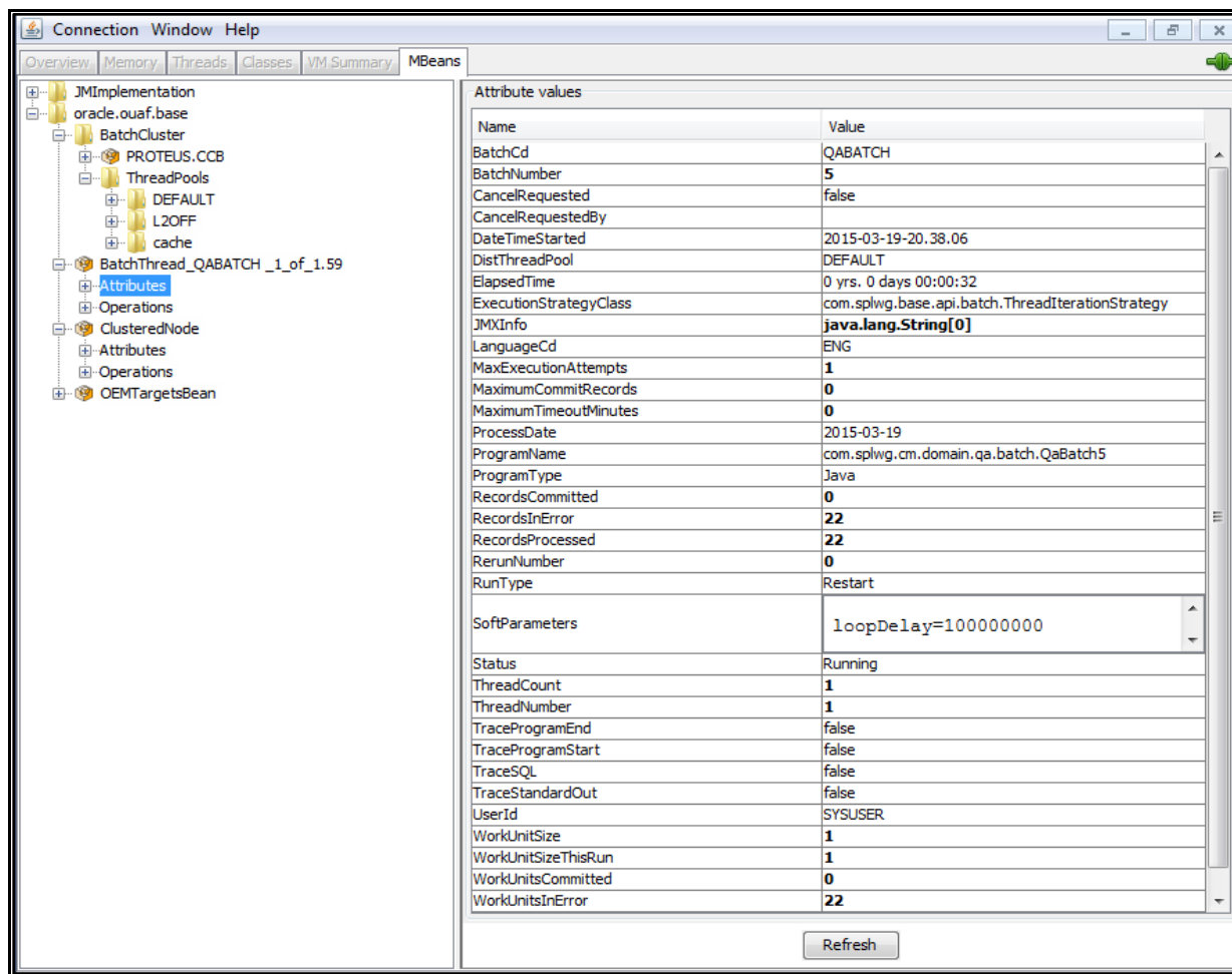
Figure 14: Batch Thread Mbean in jconsole Example
