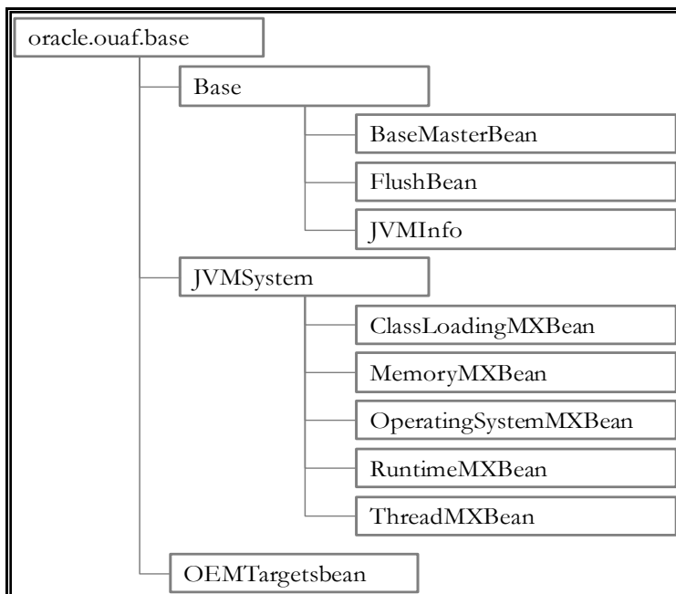
Figure 10: Web Application Server Mbeans
