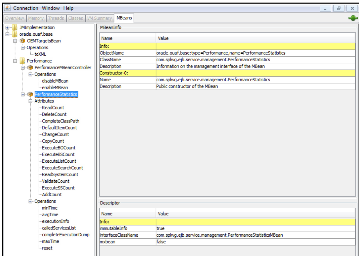
Figure 11: Business Application Server Mbeans in jconsole Example
