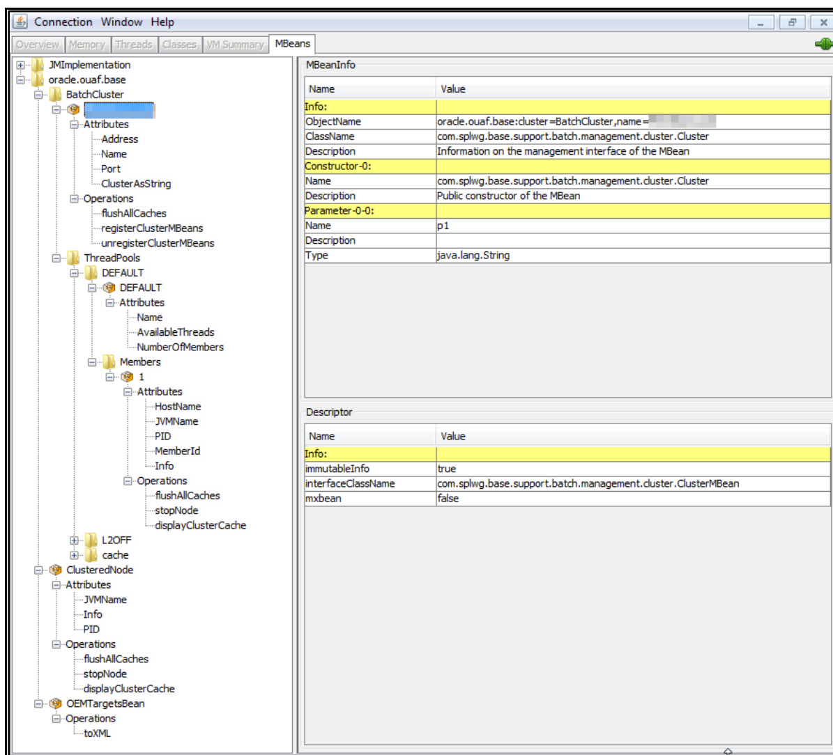
Figure 13: Batch Server Mbeans in jconsole Example
