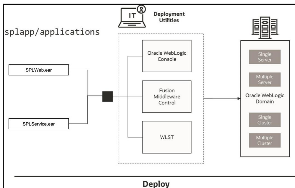
Figure 20: Web Application Server Deployment Process
