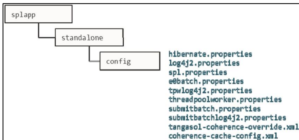
Figure 30: Batch Configuration Files
