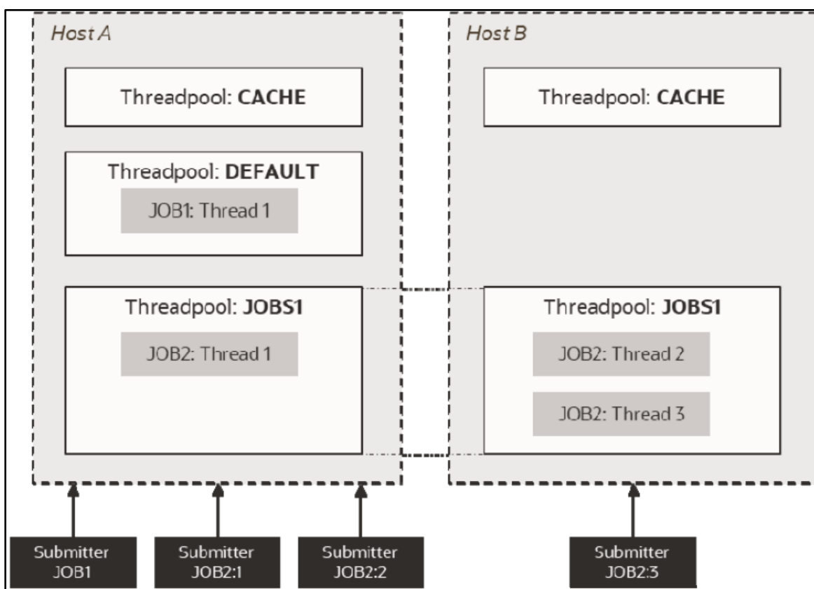
Figure 3: Batch Architecture Overview
