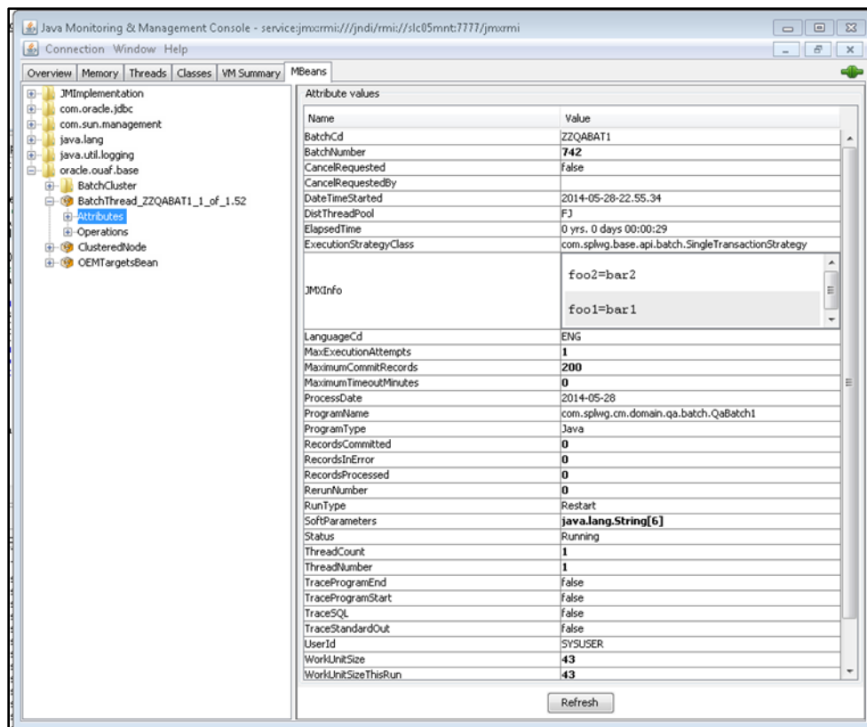
Figure 34: JMXInfo in jconsole
