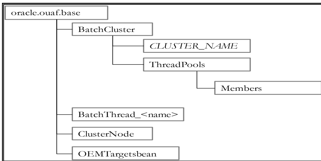
Figure 15: Batch Server Mbeans
