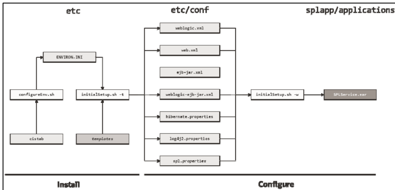
Figure 22: Business Application Server Configuration Process
