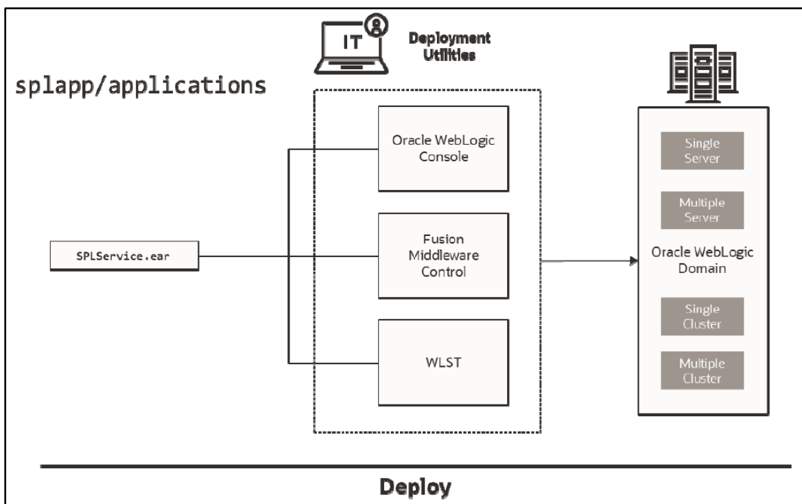
Figure 24: Business Application Server Deployment Process
