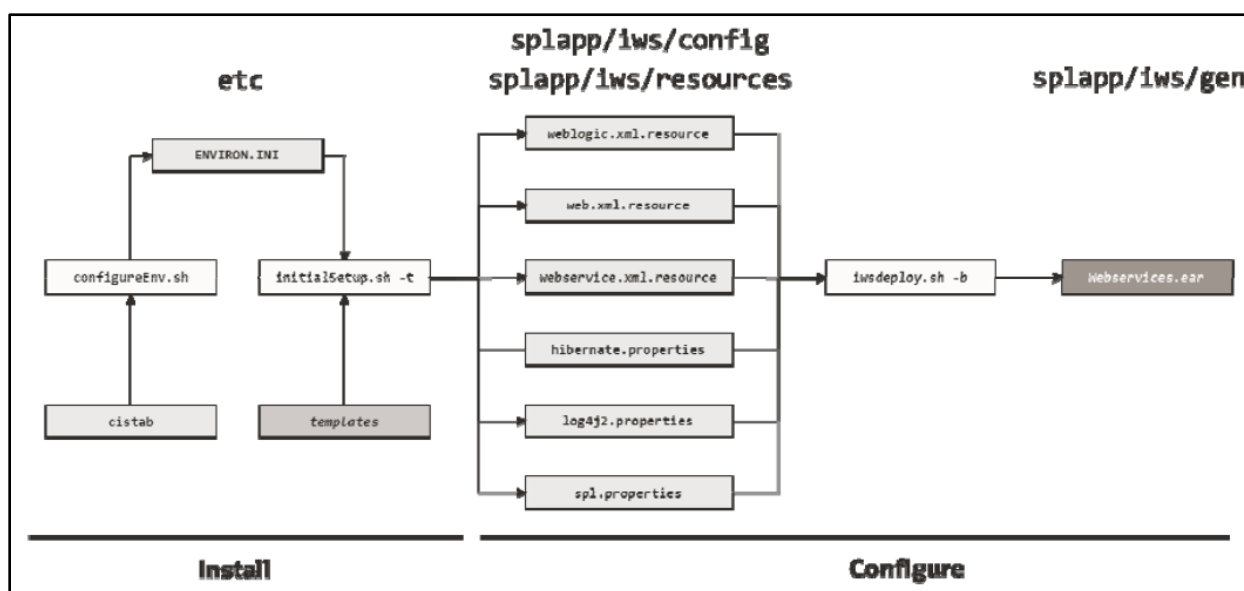
Figure 27: Inbound Web Services Configuration Process
