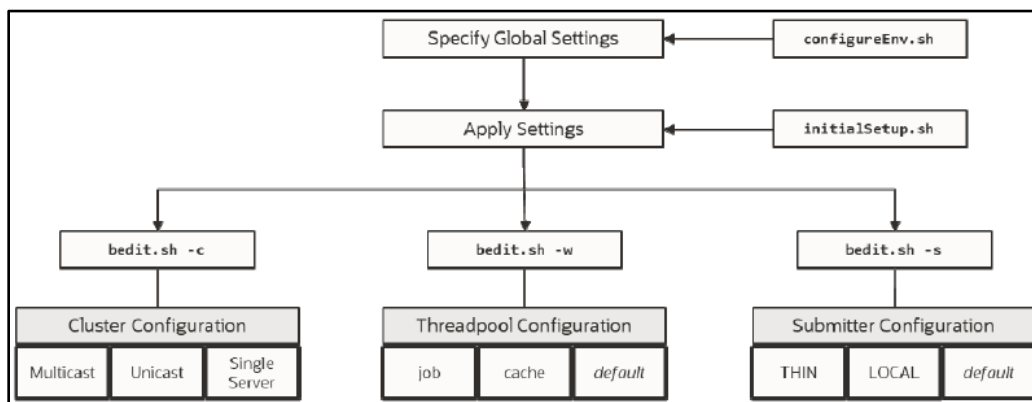
Figure 32: bedit Configuration Process
