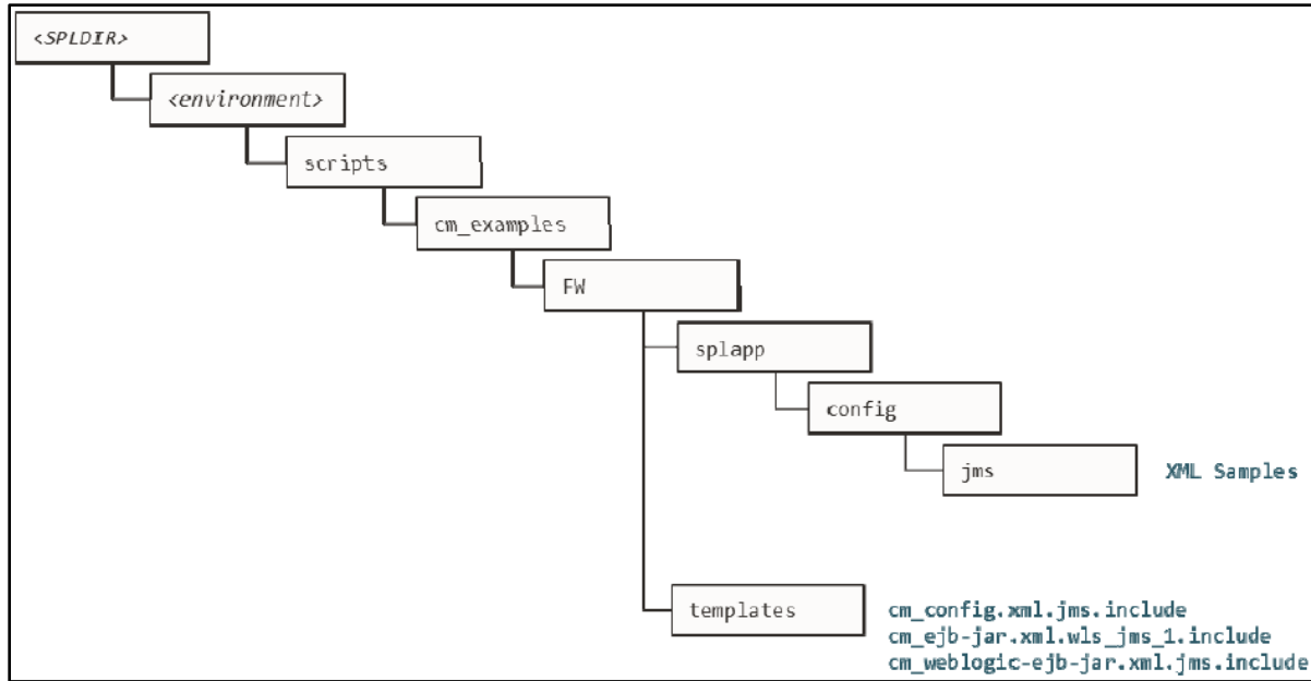
Figure 38: Custom JMS Configuration
