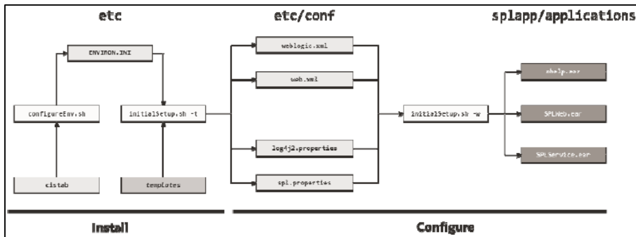
Figure 19: Web Application Server Configuration Process
