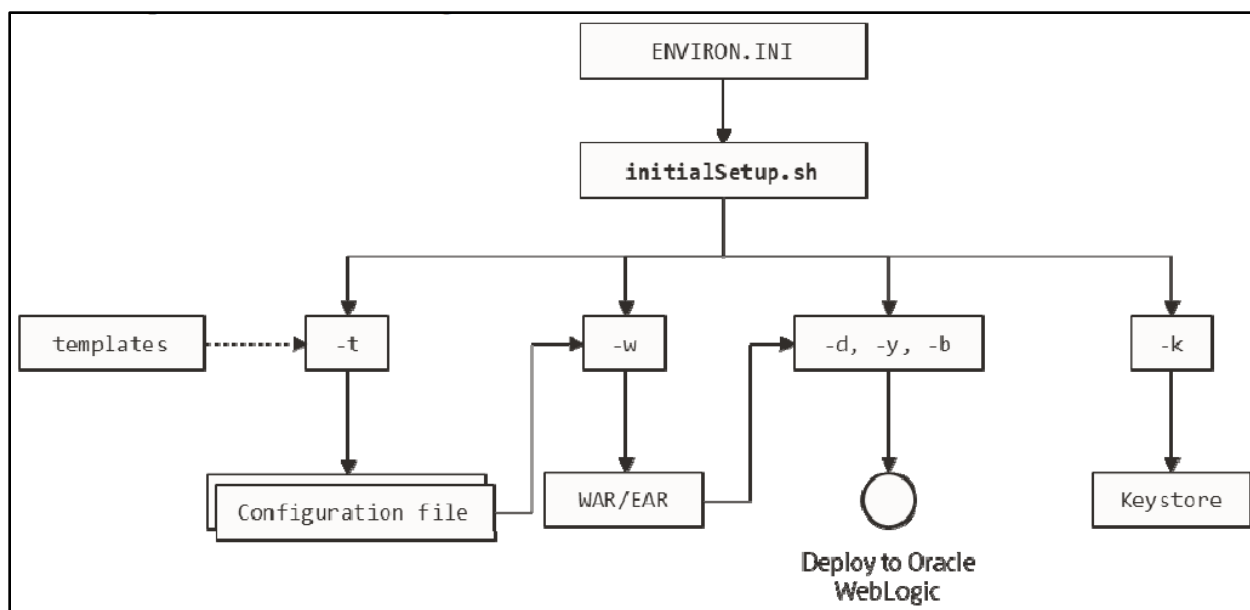
Figure 5: initialSetup Command Structure
