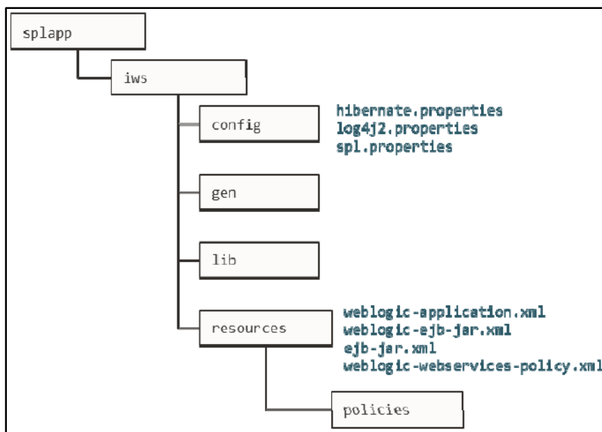
Figure 26: Inbound Web Services Structures
