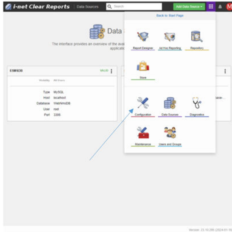
Figure 10-38 Configuration Card
