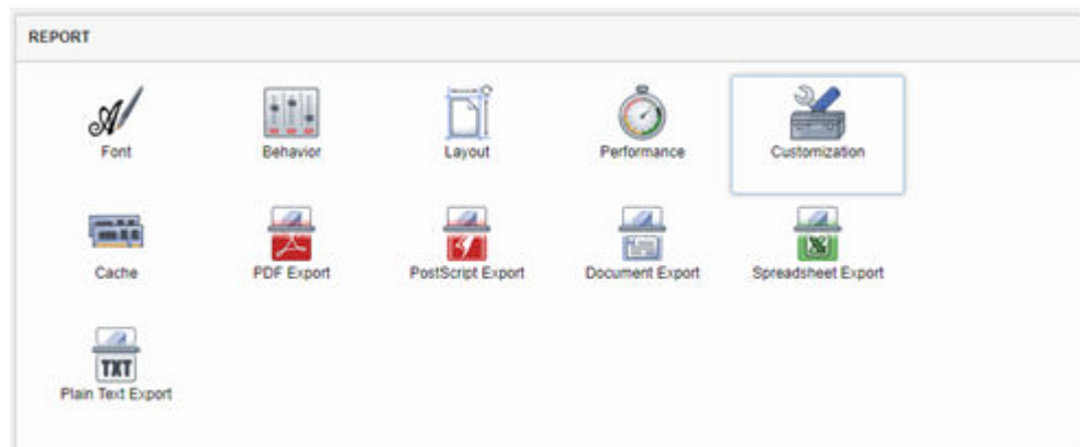
Figure 10-47 Report section
