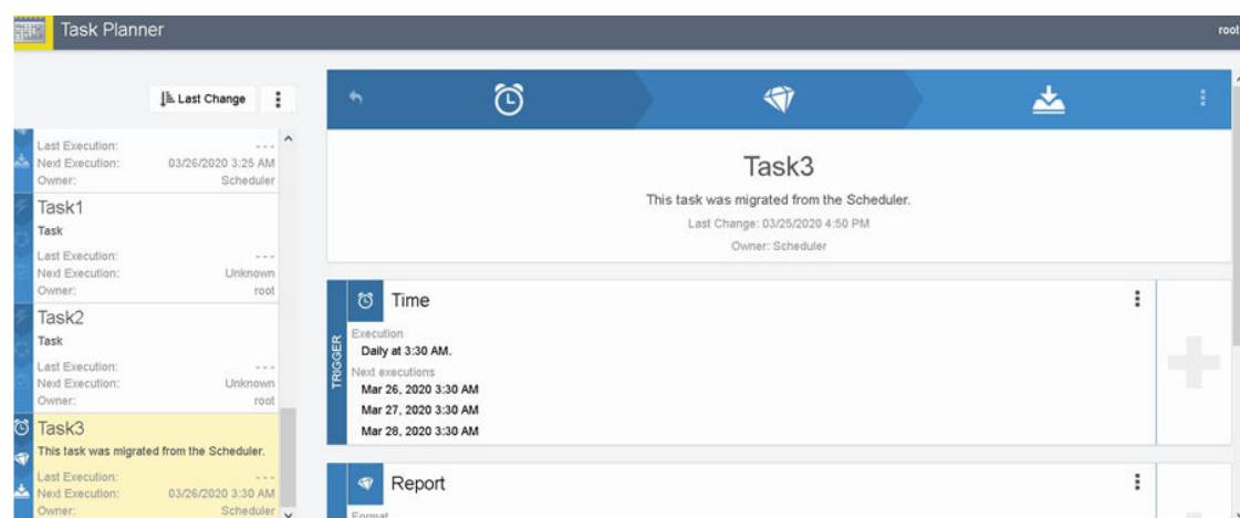
Figure 10-11 Task Planner
