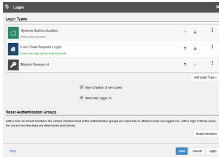
Figure 10-62 Login pop-up
