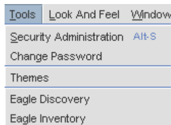
Figure 5-1 EAGLE Discovery
