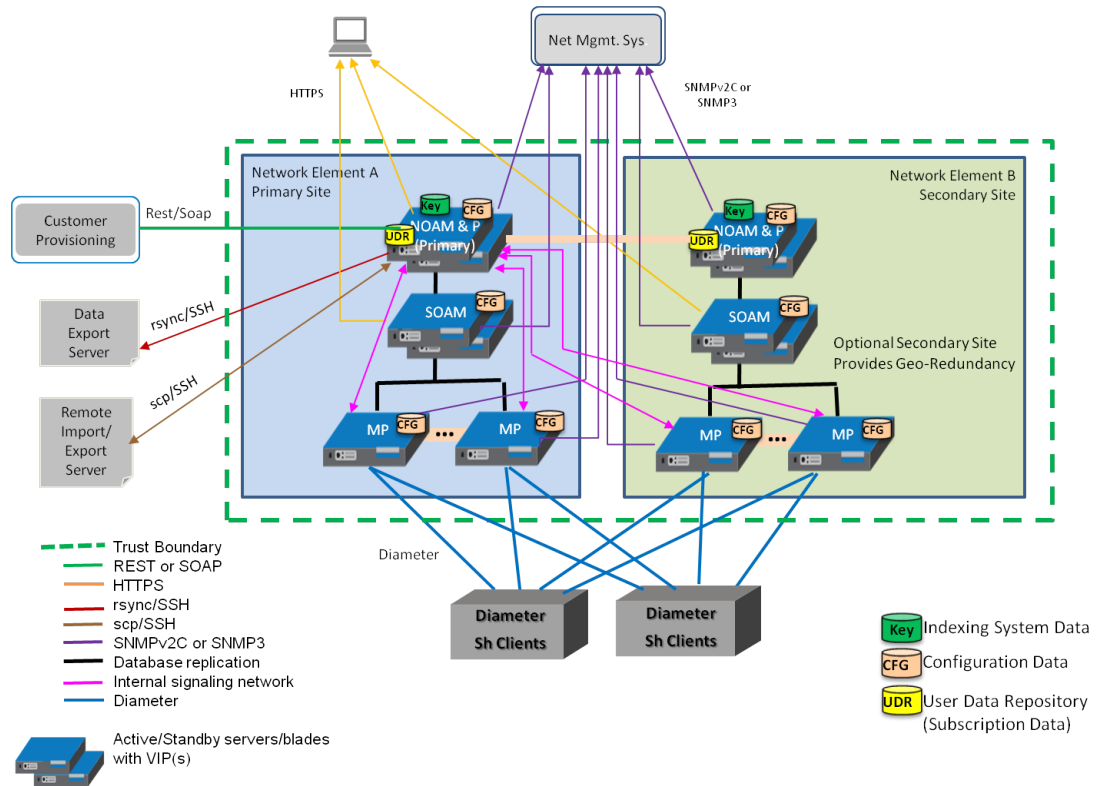
Figure 3-1 UDR System Architecture
