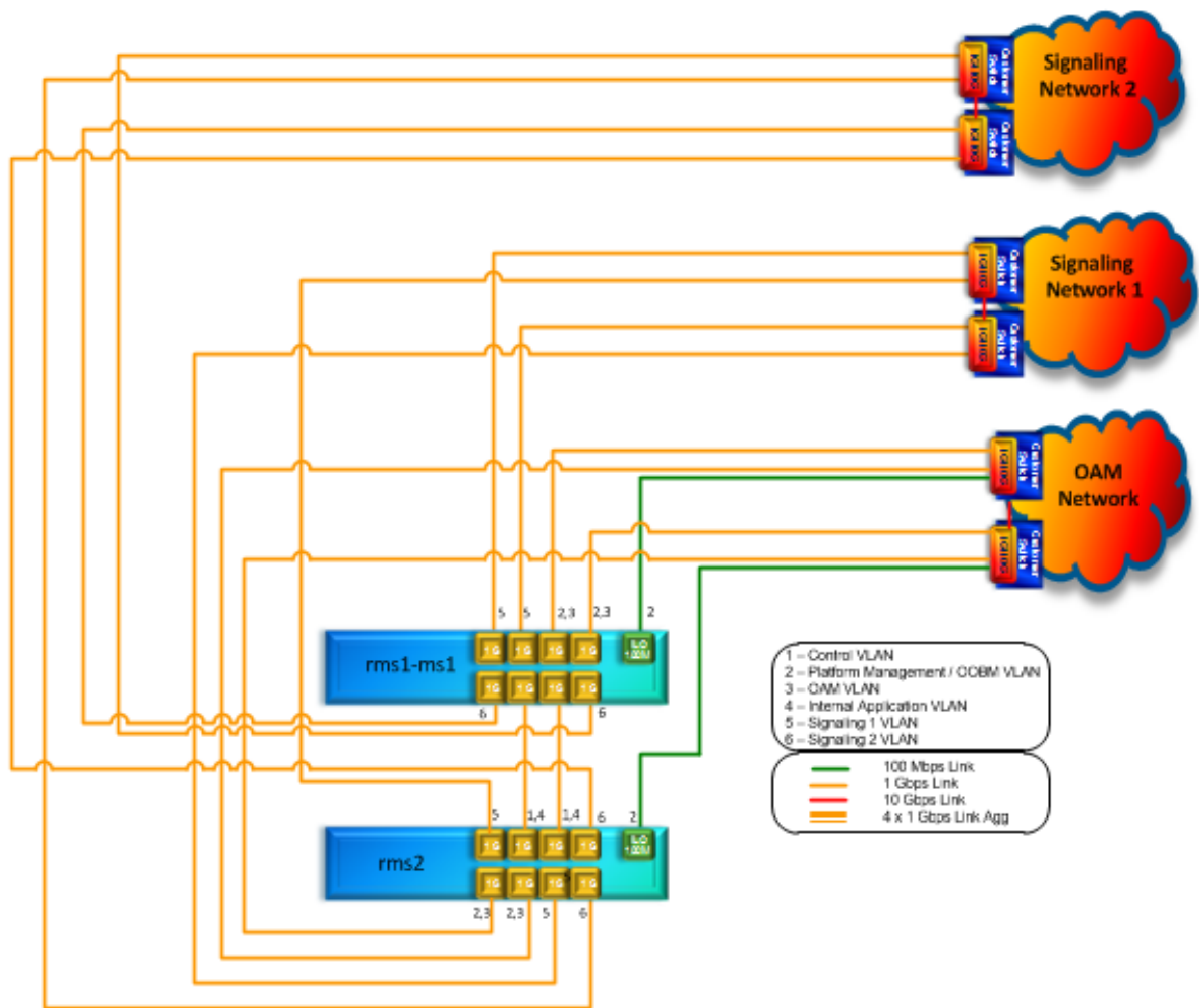
Figure 9: Logical Diagram Topology 7E
