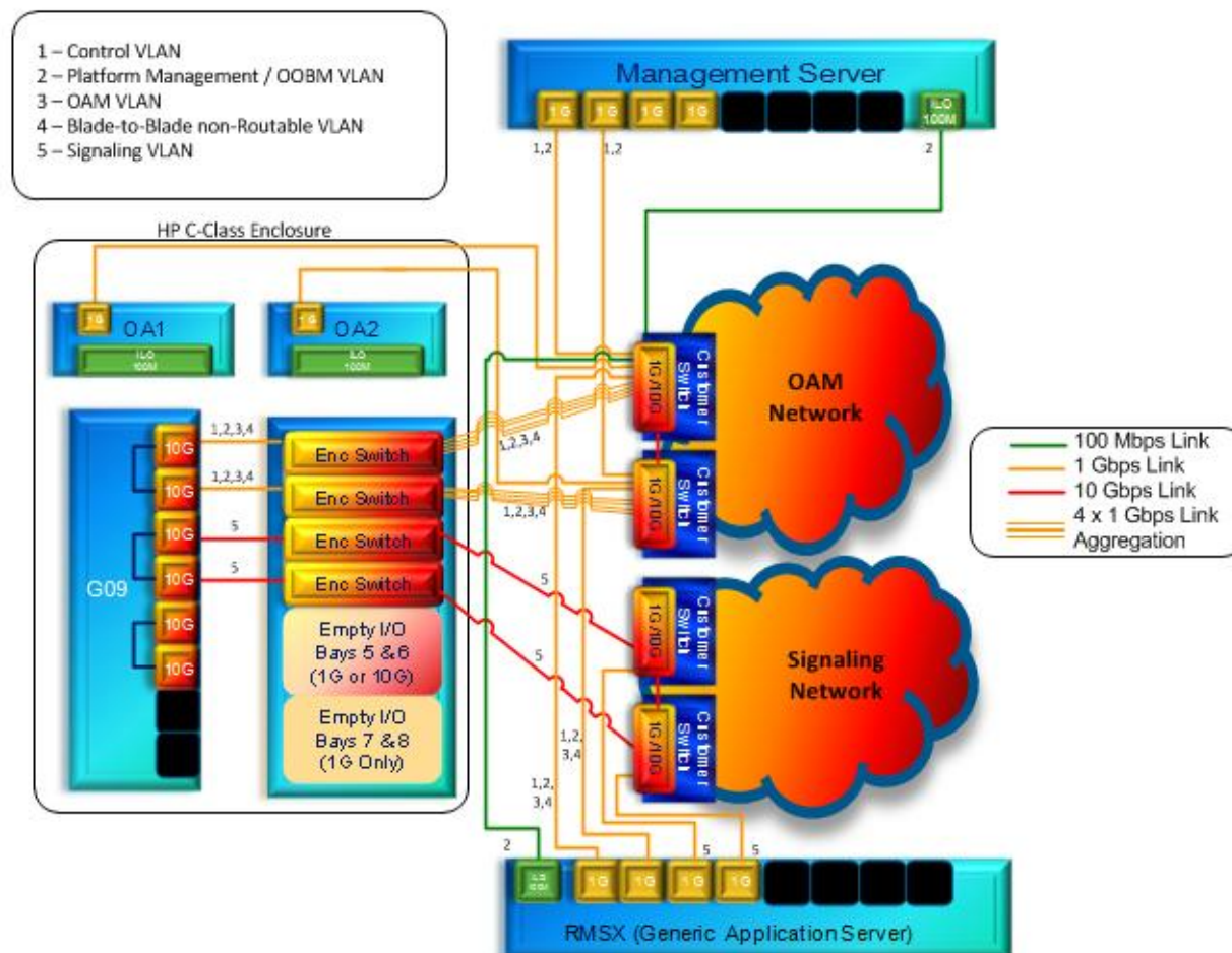
Figure 6: Logical Diagram Topology 4
