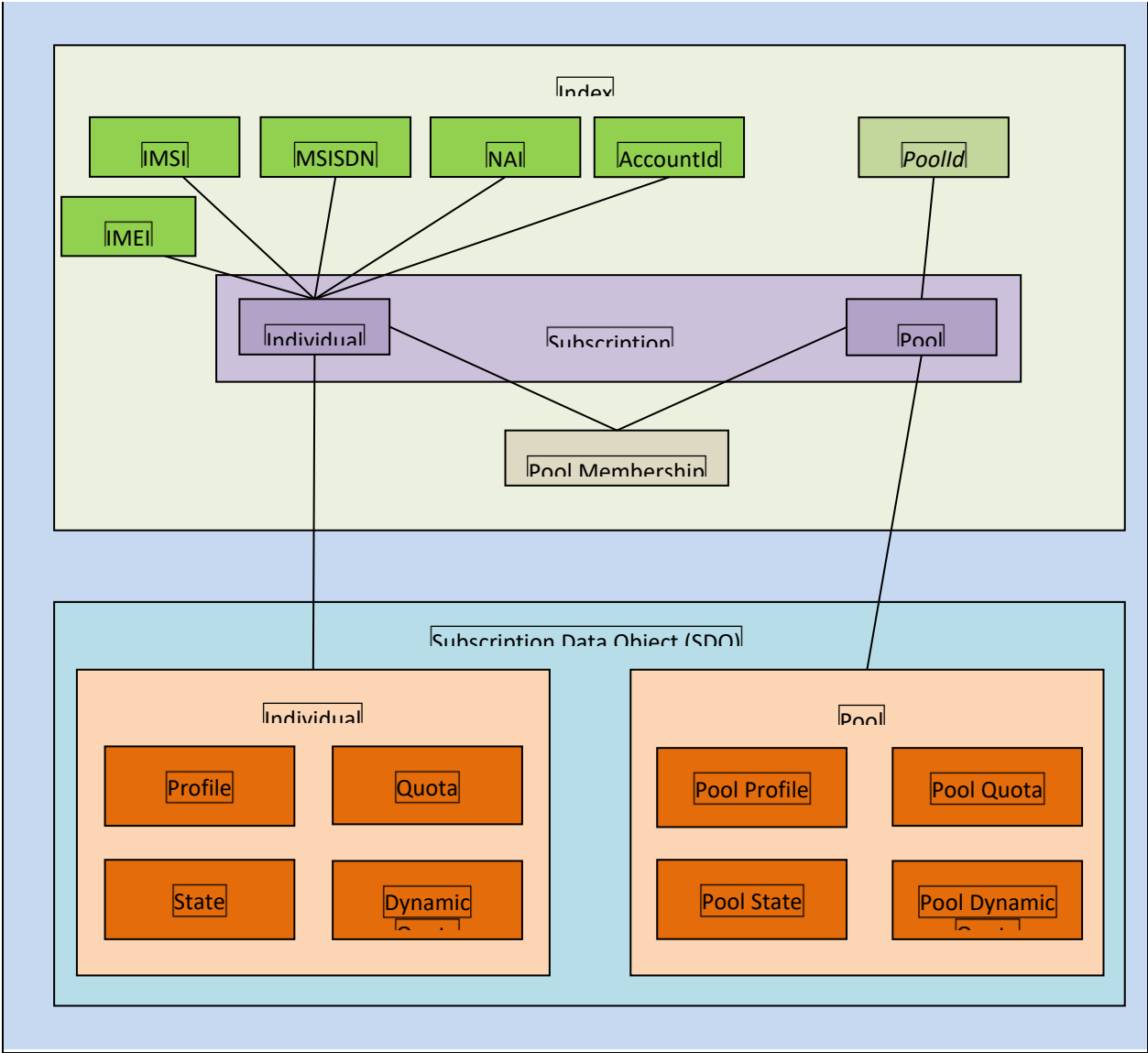
Figure 2: Data Model
