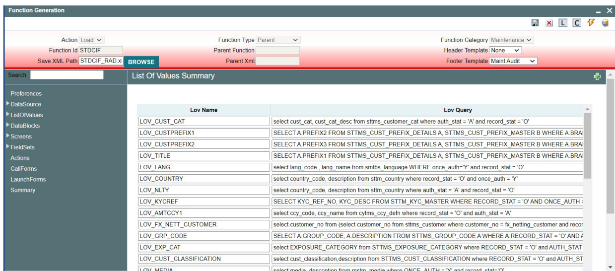
Fig 11.1 Adding a new LOV
