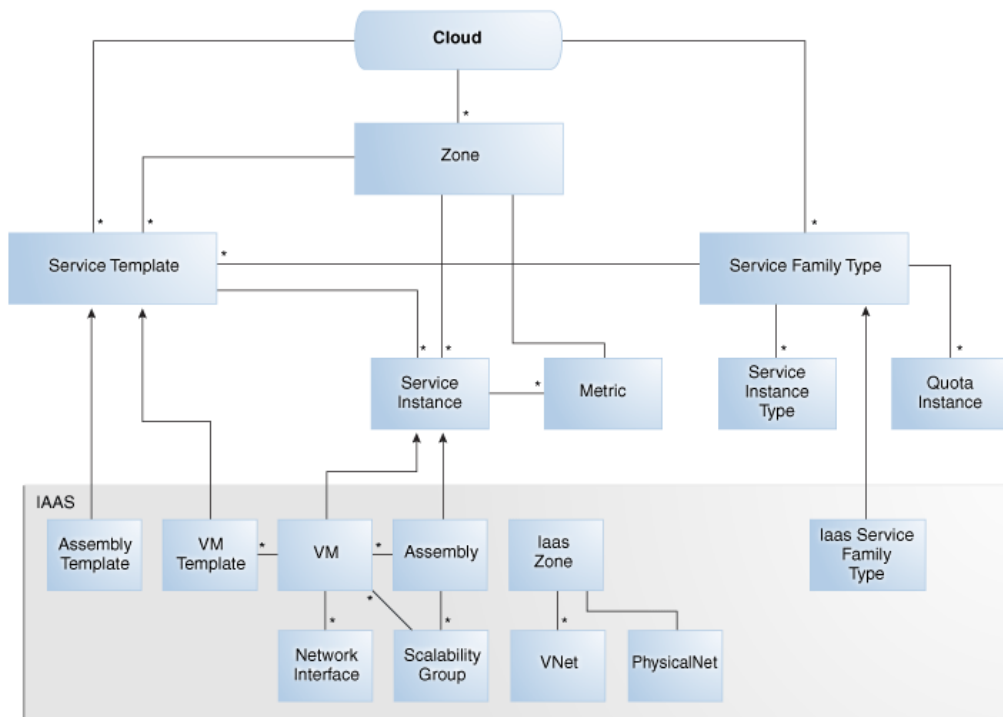
Figure 66-1 IaaS Resource Model
