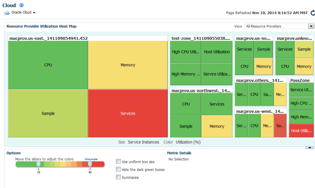
Figure 40-2 Resource Provider Utilization Heat Map
