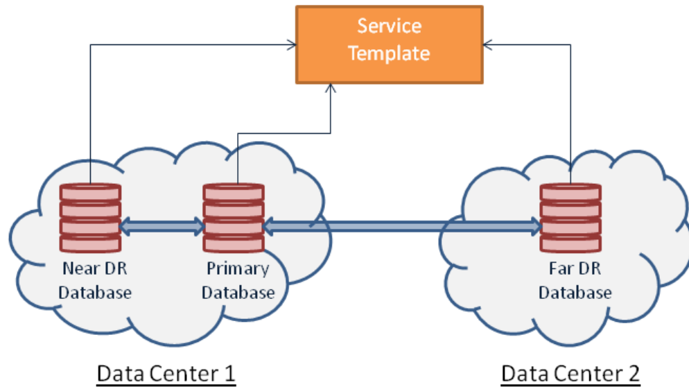
Figure 57-2 Multi-Datacenter DBaaS Setup
