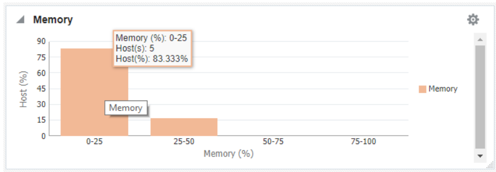
Figure 45-6 Memory Graph
