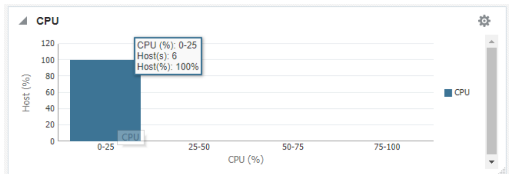
Figure 45-4 CPU Graph
