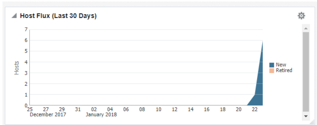
Figure 45-3 Host Flux
