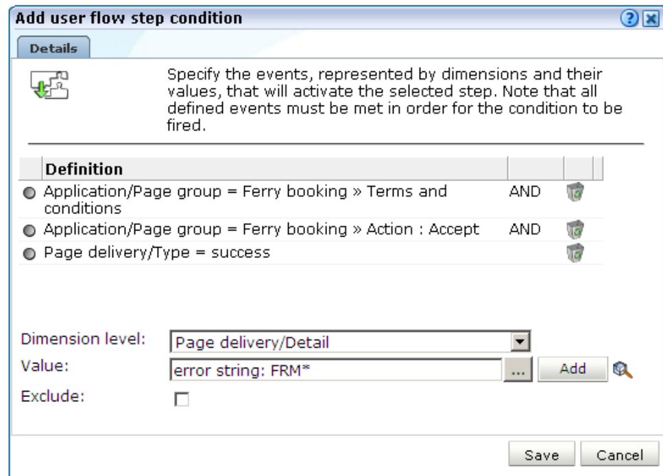
Figure 9-3 Add User Flow Step Condition
