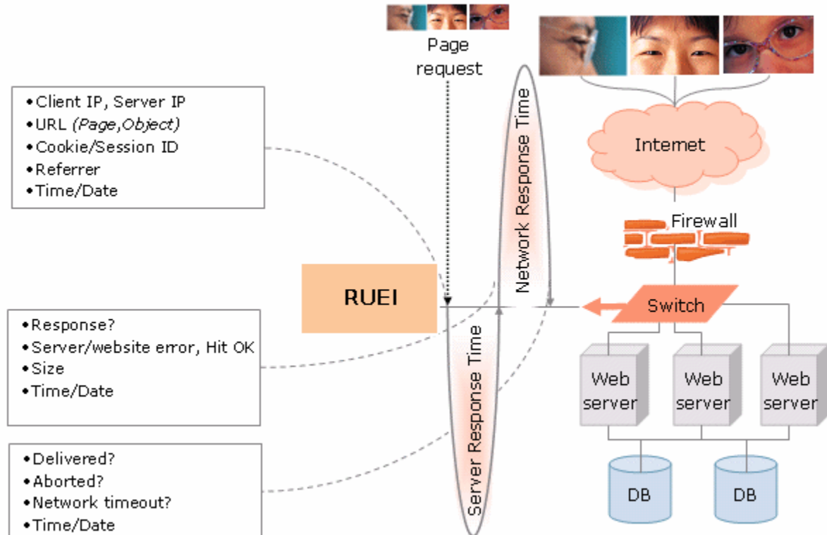
Figure E-1 RUEI Data Monitoring
