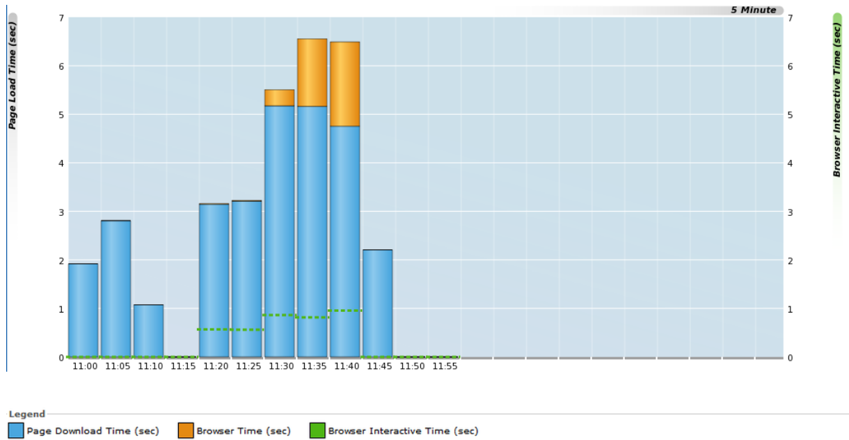
Figure 12-34 Page Loading Time Breakdown View
