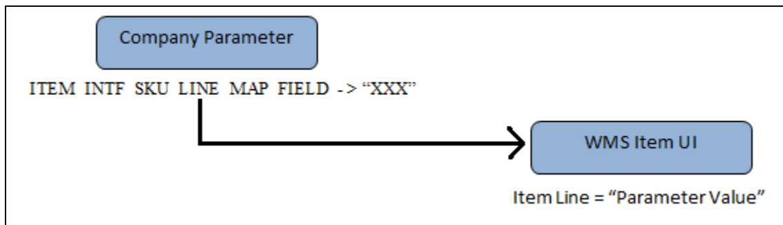
Figure 3-3-2: UI – SKU_LINE
