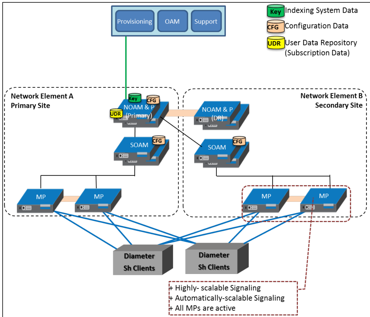
Figure 1: UDR High Level Architecture
