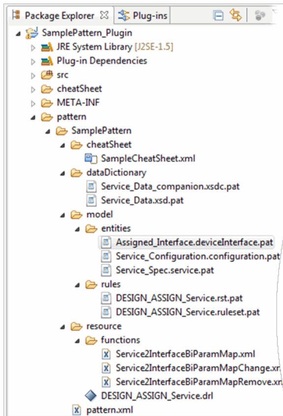
Figure 2–2 Design Pattern Folder Structure Example
