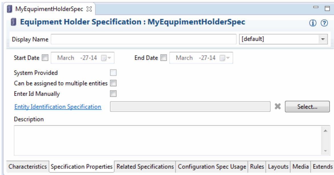
Figure 2–9 Specification Editor: Enter Id Manually Deselected
