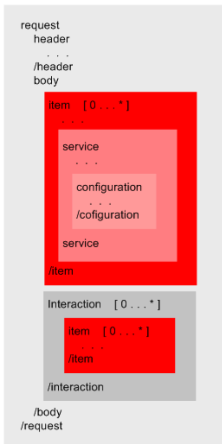
Figure 2–3 Request Content
