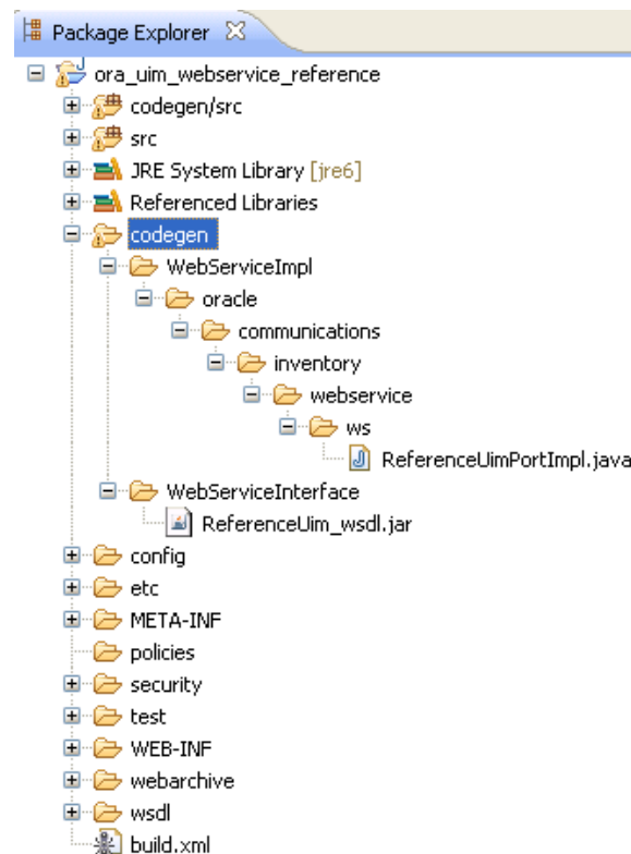
Figure 4–10 Package Explorer View Including the codegen Directory Generated Files
