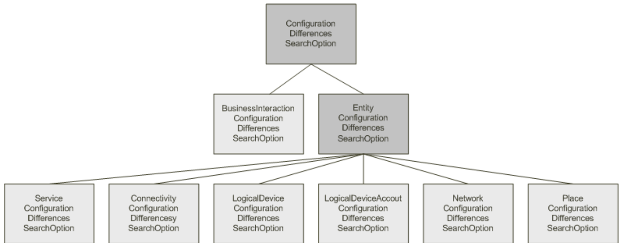
Figure 2–11 Search Options
