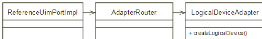
Figure 4–7 Implementation Pattern
