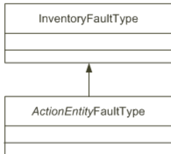
Figure 4–4 Fault Types
