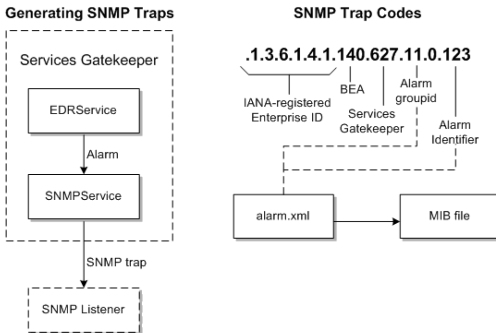
Figure 10–1 SNMP Overview
