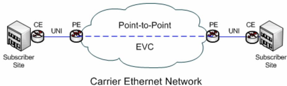
Figure 12–1 Point-to-point EVC
