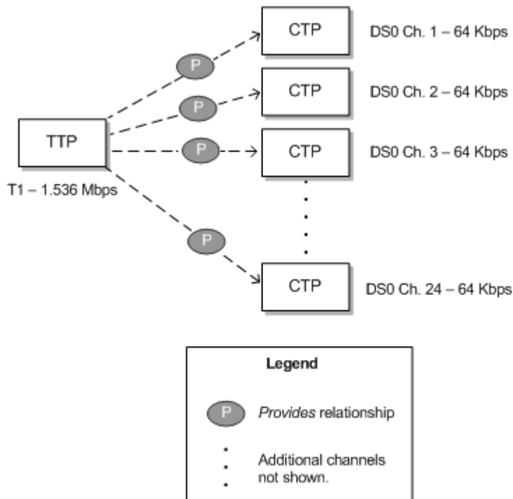
Figure 17-7 Simple Signal Structure
