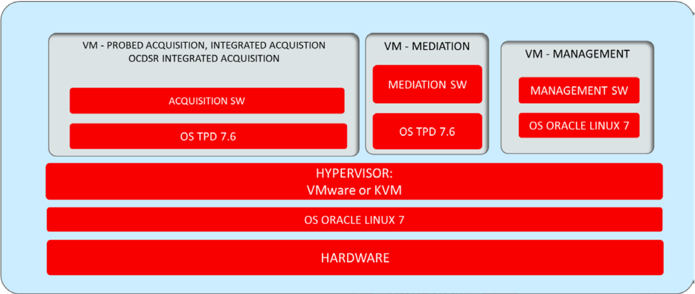
Figure 18 – Performance Intelligence Center Virtualization configurations
