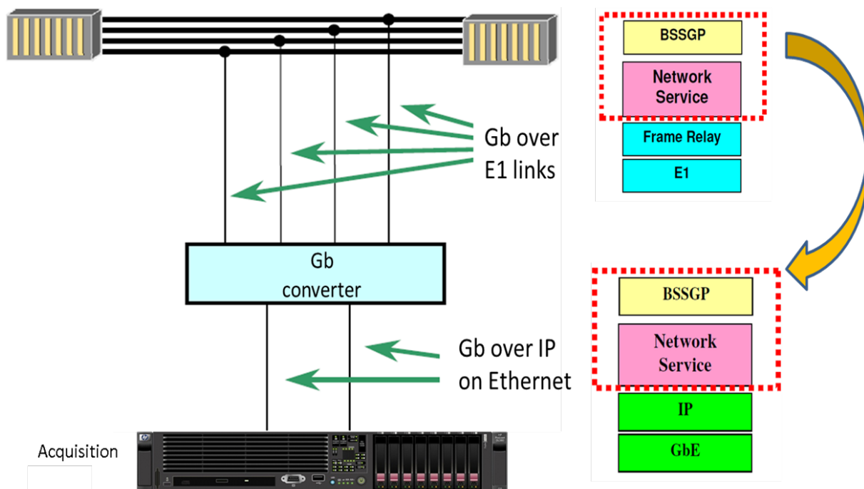
Figure 6 – GboE1 to GboIP Converters – layers
