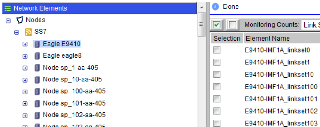
Figure 31 : Linkset Display
