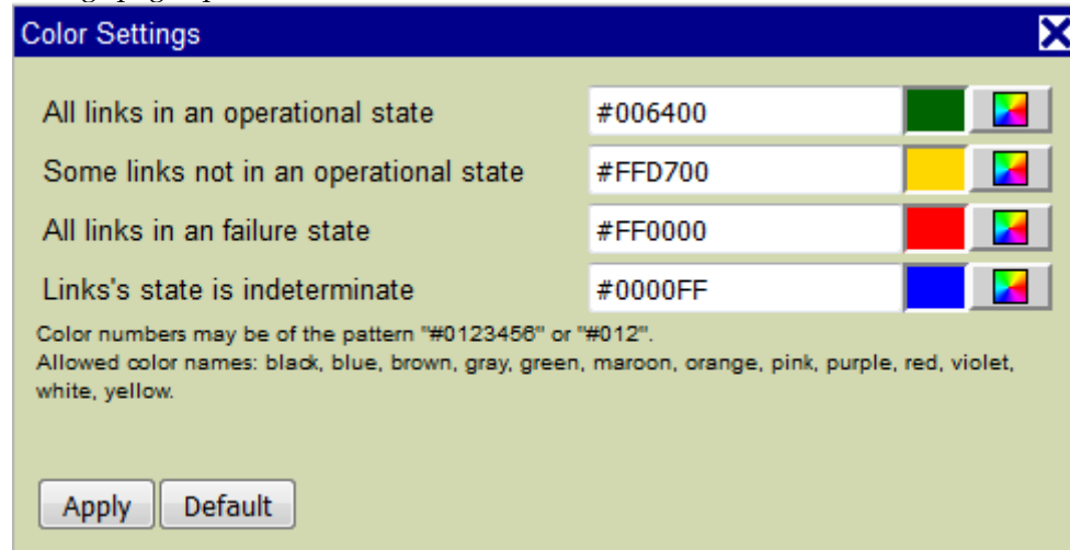
Figure 36 : Color Settings
