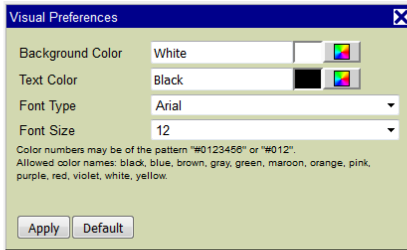
Figure 38 : Visual Preferences
