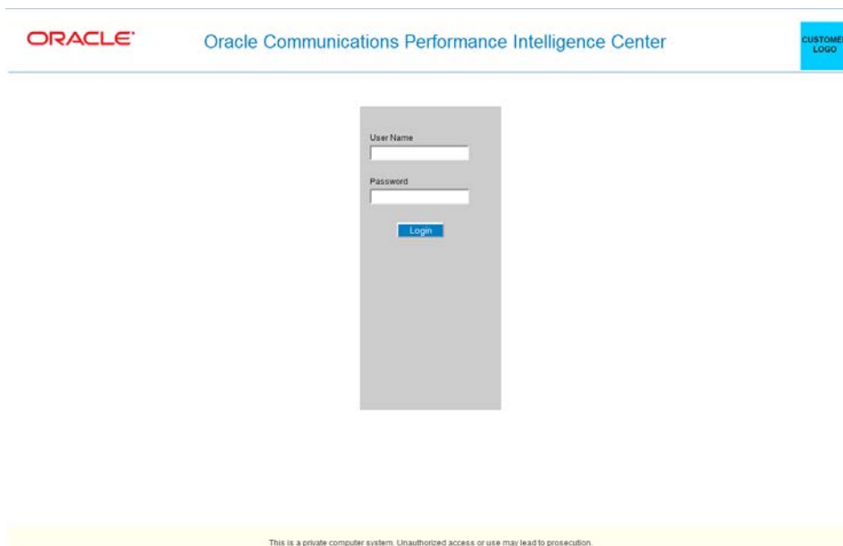
Figure 1 : Login Screen
