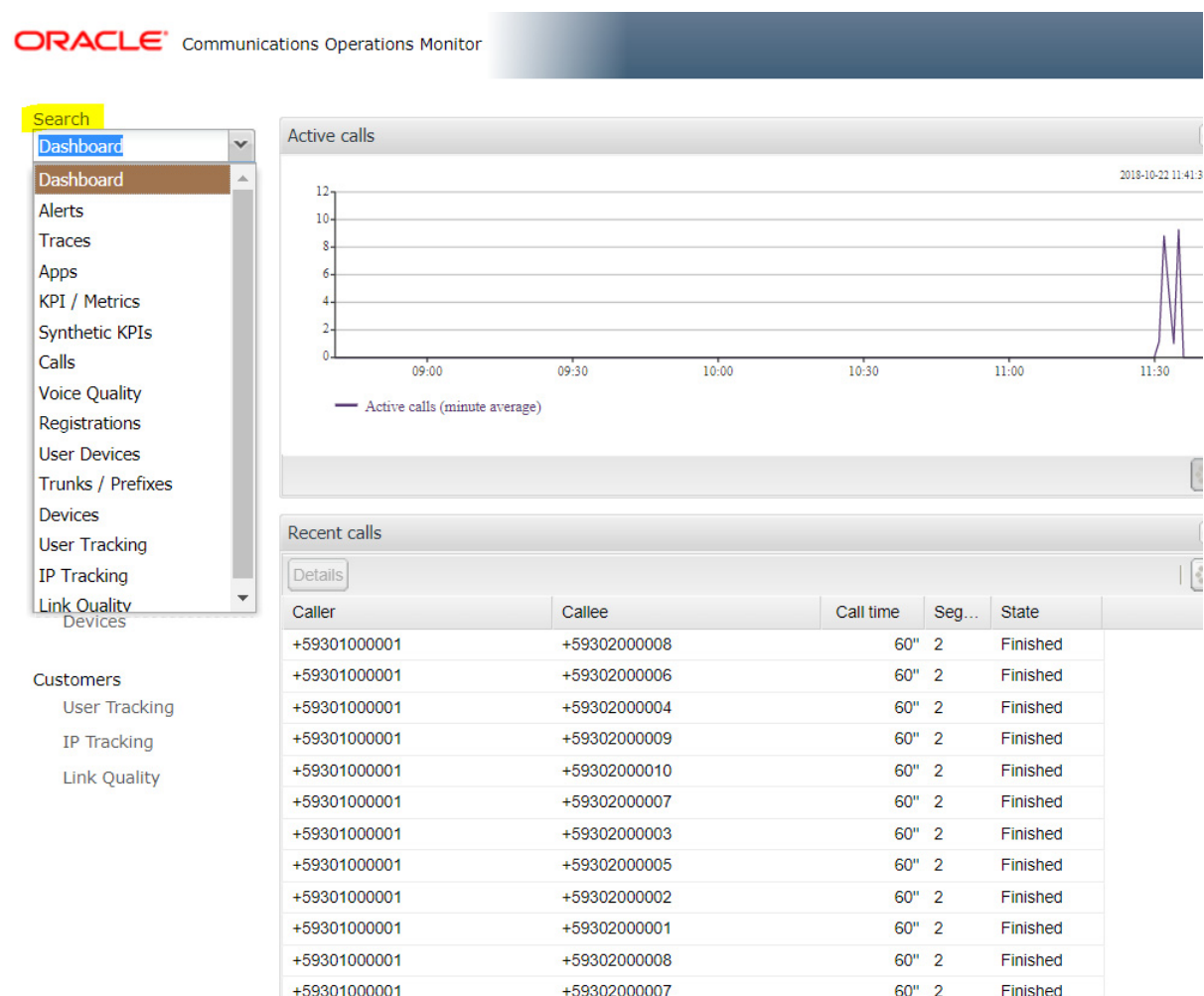
Figure 3–11 Dashboard
