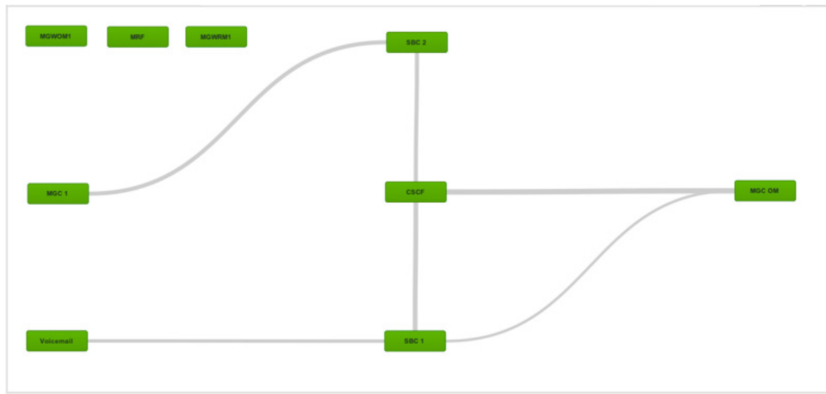
Figure 4-64 Device Map
