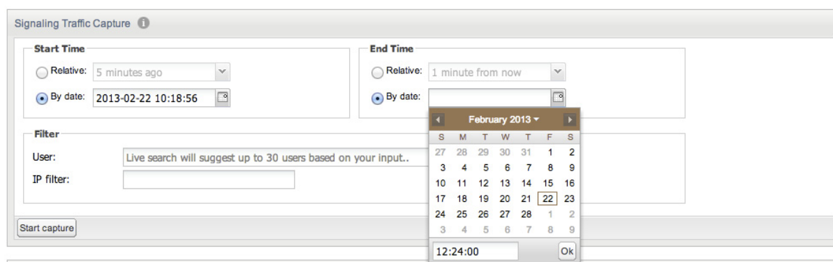
Figure 3–24 Trace Example 1
