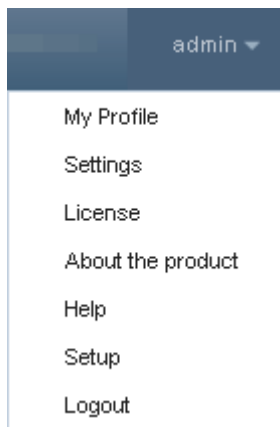
Figure 3–1 User Menu
