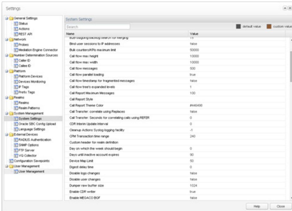
Figure 2–2 System Settings
