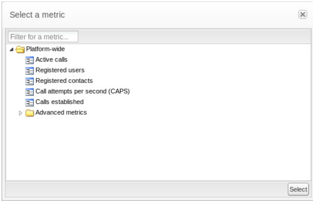
Figure 3–19 Metrics Dialog
