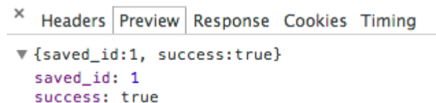
Figure 11–10 Preview Tab
