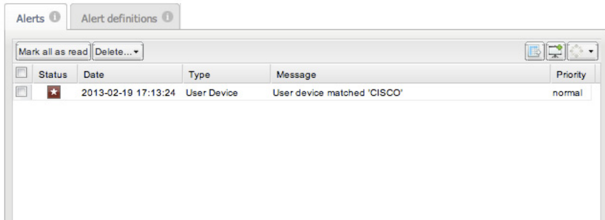
Figure 3–13 Alerts Table
