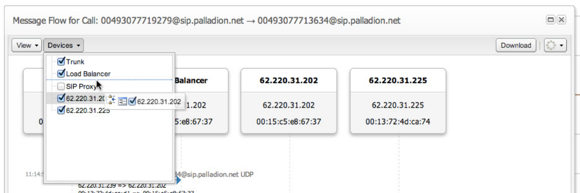
Figure 3-10 Devices Menu
