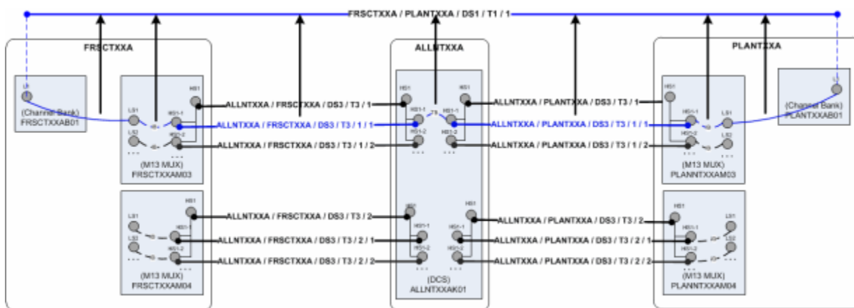
Figure 14-27 2:2 Inter-Facility Grooming: Before
