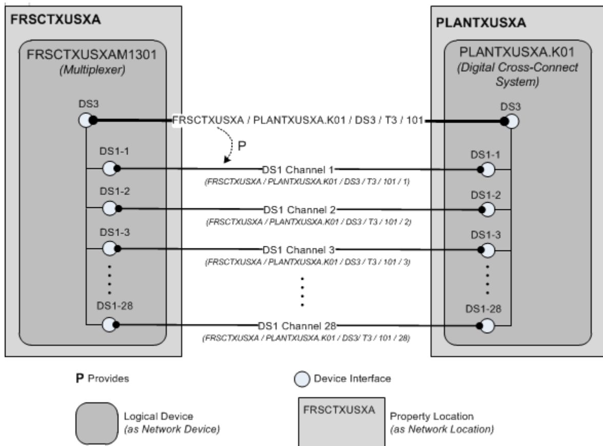
Figure 14-2 Channel Termination
