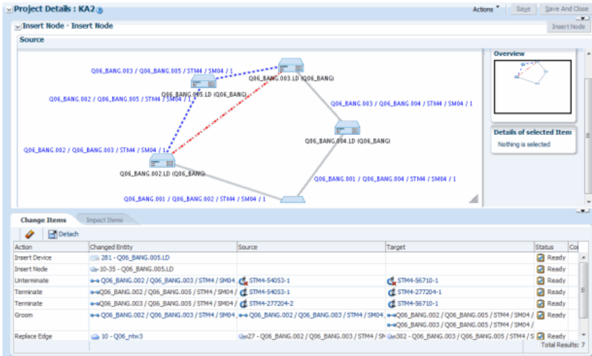
Figure 14-43 UIM Insert Node User Interface - After Activity Configuration
