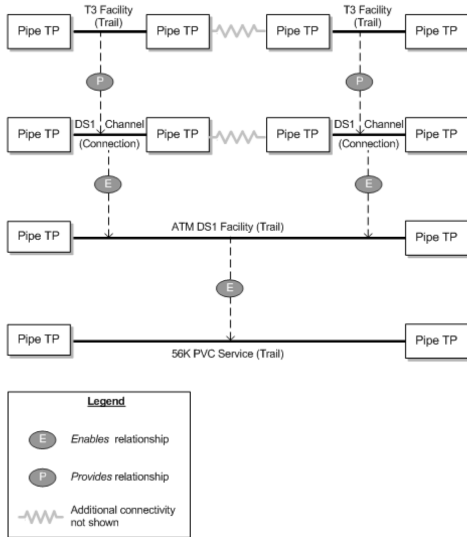
Figure 17-6 Trail and Connection Pipes
