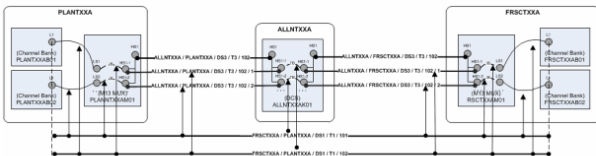
Figure 14-40 Network Node Insertion: After
