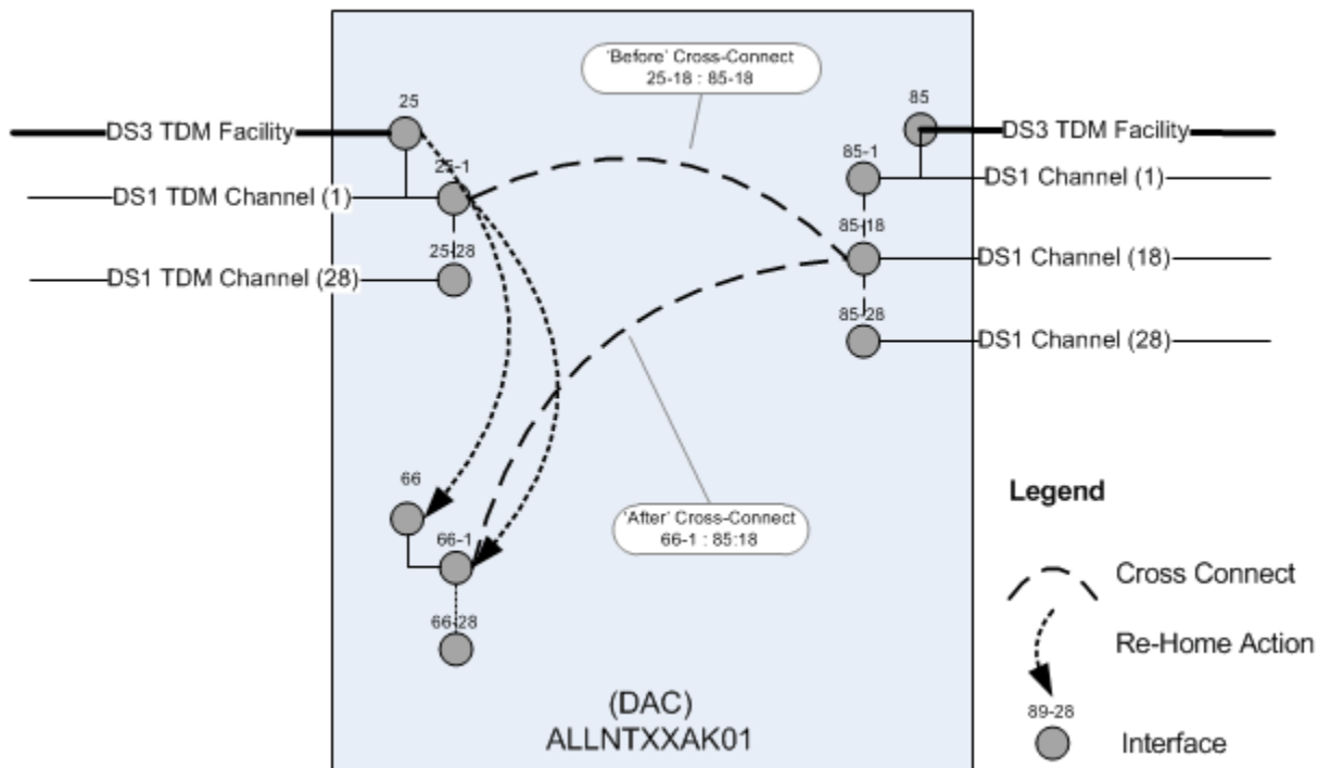
Figure 14-33 Rehoming Impact on Cross-Connects
