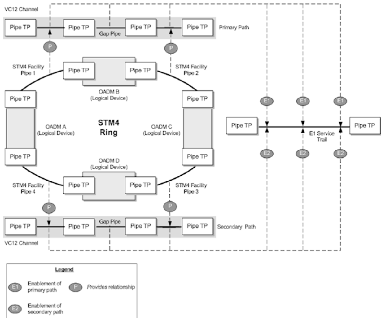
Figure 17-5 Multiple Enablement of an E1 Service Trail
