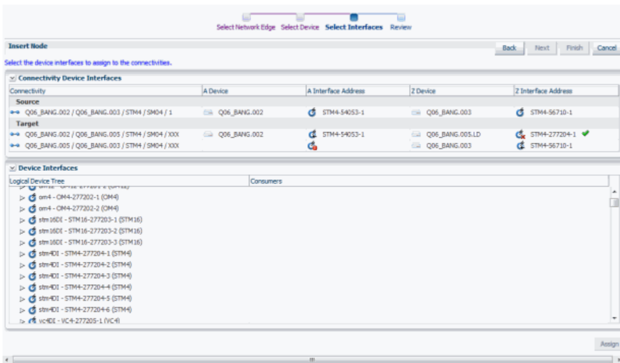
Figure 14-41 Select Interfaces Area of the Insert Node Dialog Box
