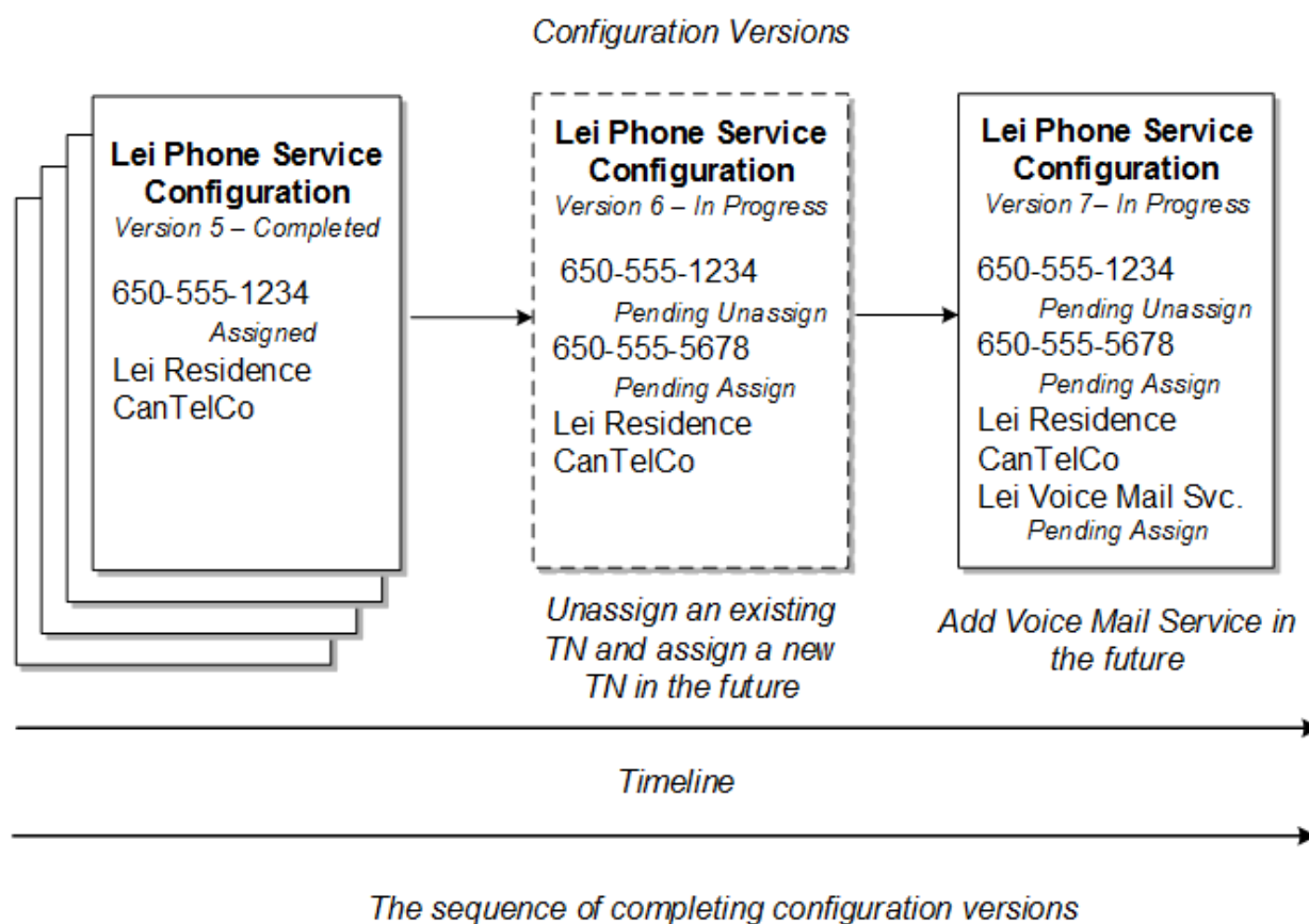
Figure 5-8 Sequence of Completing Configuration Versions
