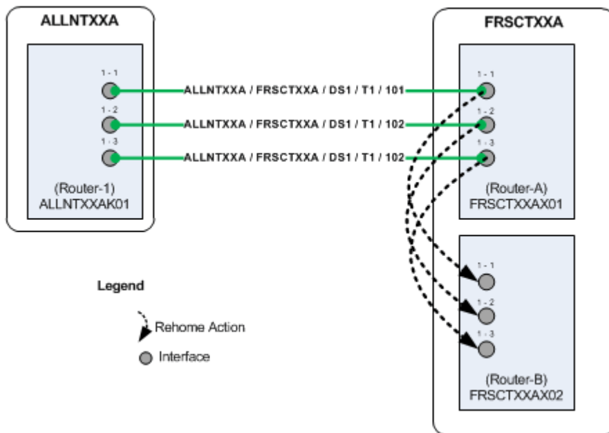
Figure 14-32 Simple Rehoming Scenario
