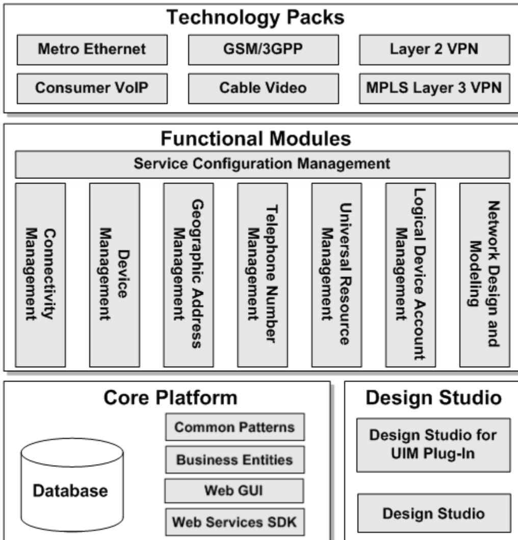
Figure 1-1 UIM Components
