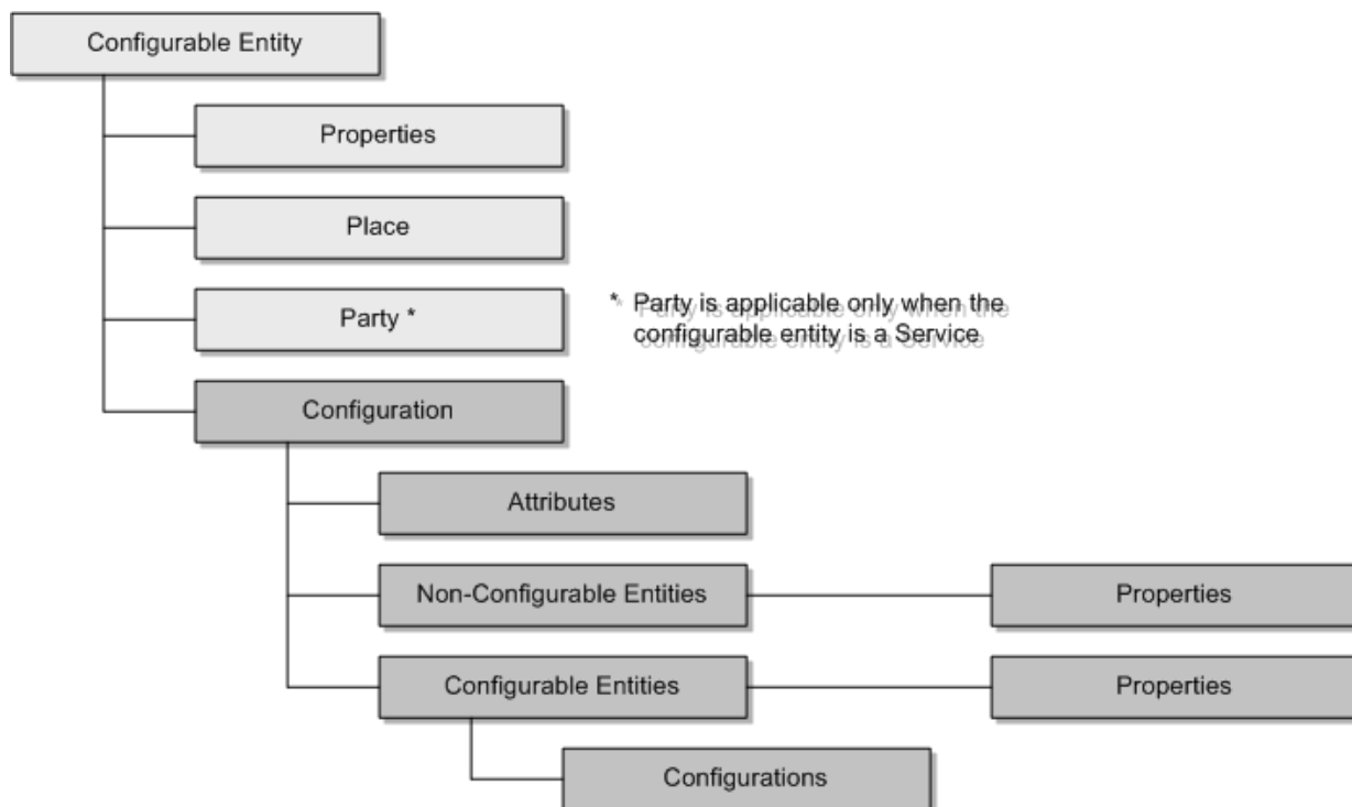
Figure 2-8 Example Service Configuration Retrieval
