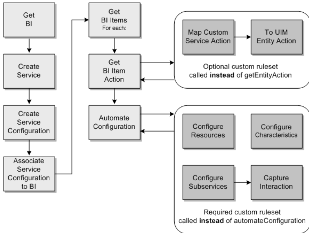
Figure 2-4 ProcessInteraction Logic Flow
