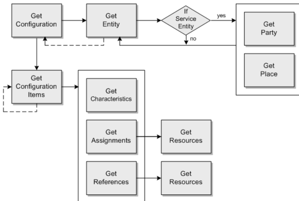
Figure 2-9 GetConfiguration Logic Flow
