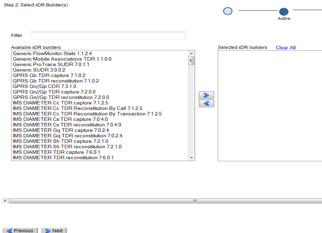
Figure 164: Dataflow Assistant for Mediation Protocol Selection
