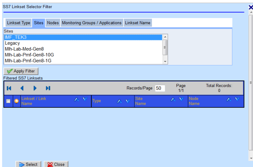
Figure 80: Sites Screen
