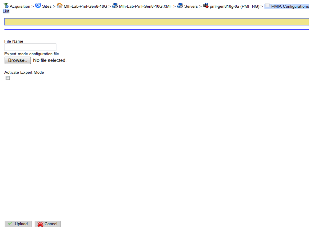
Figure 101: PMIA Screen
