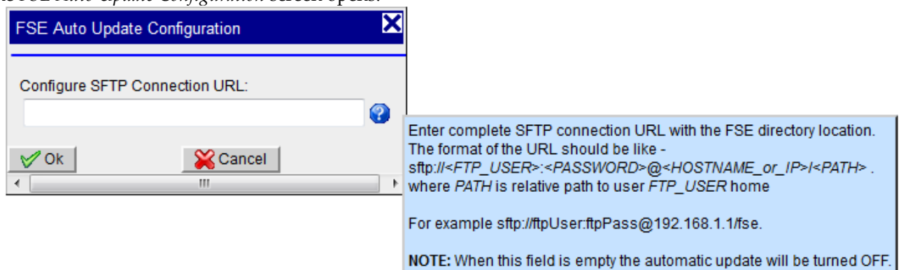
Figure 268: FSE automated update configuration screen
