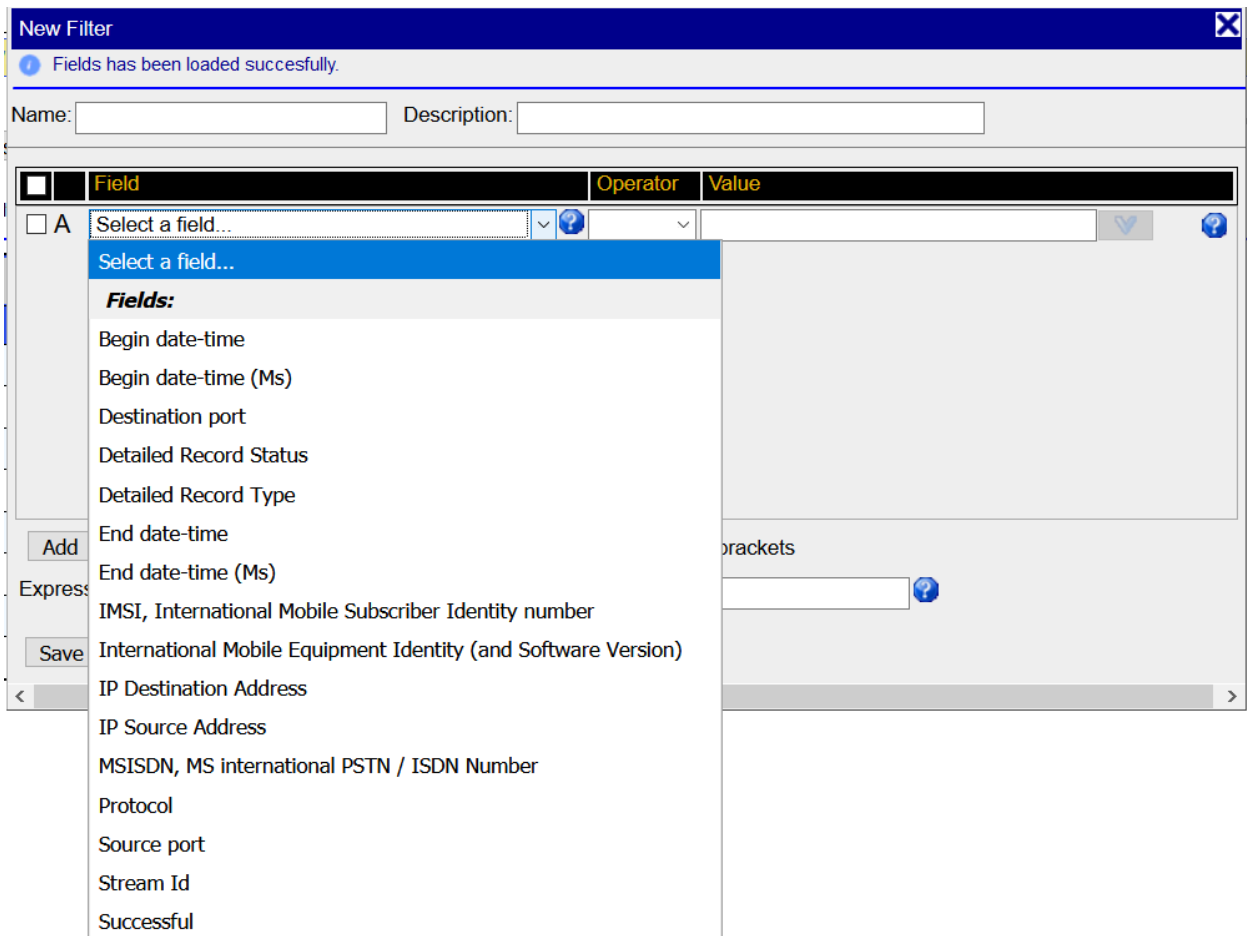
Figure 14: Fields in apply filter – xDR Reduced Field session
