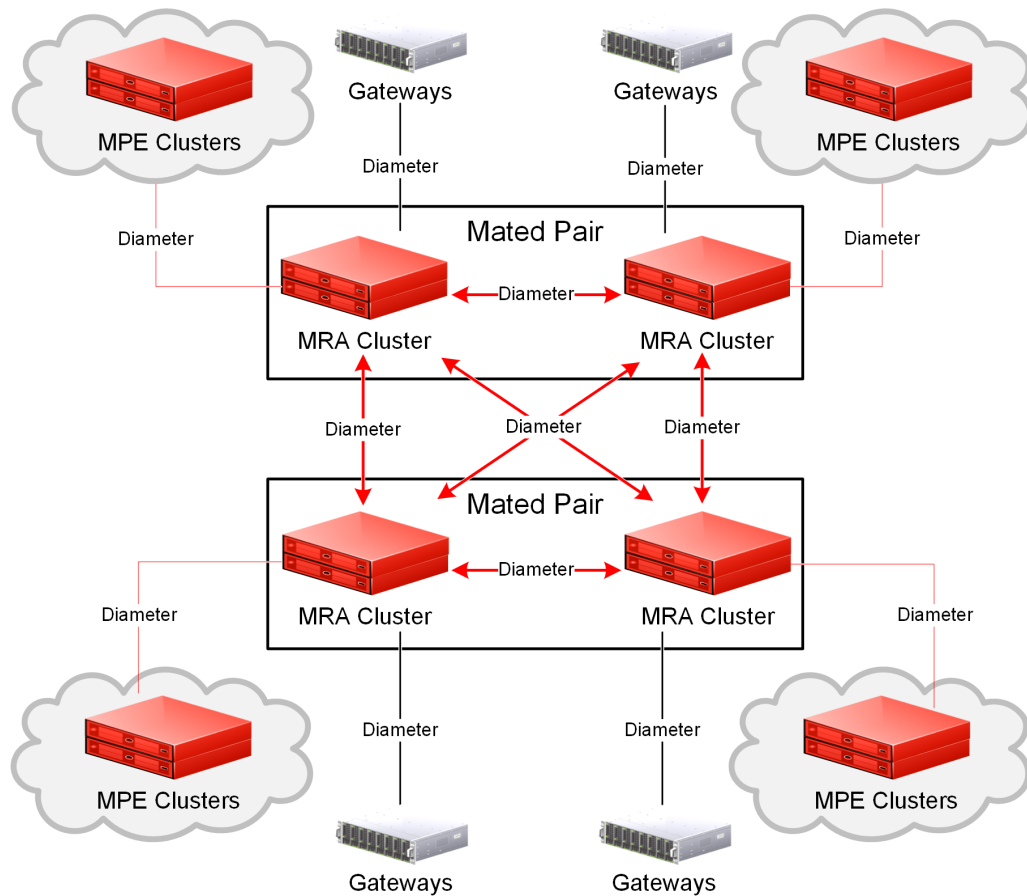
Figure 1-1 Typical MRA Network
