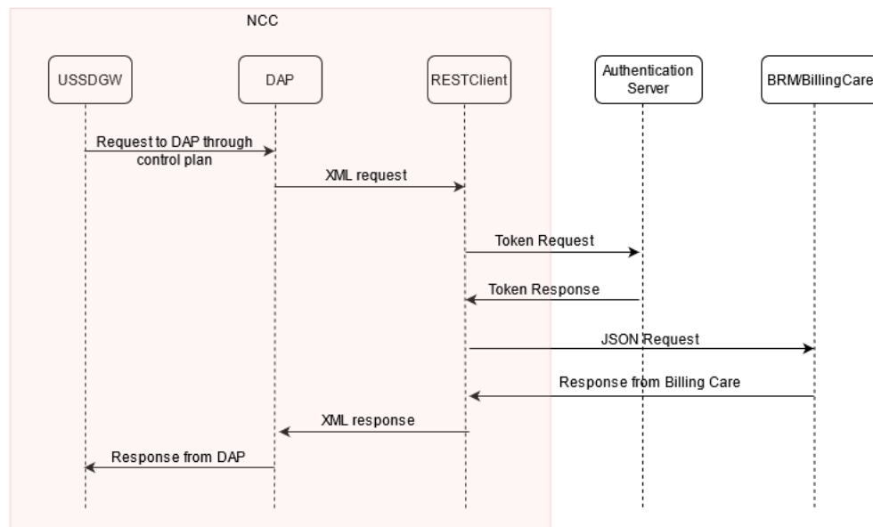
Figure 5-1 REST Request Flow
