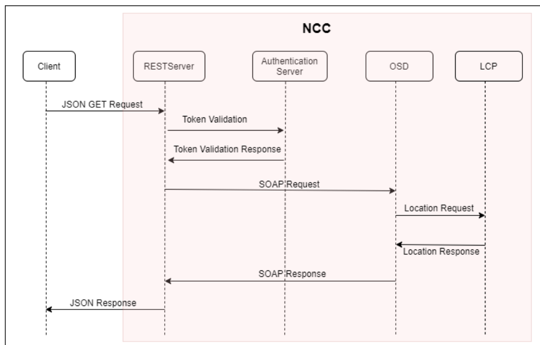
Figure 11-1 RESTServer Call Flow
