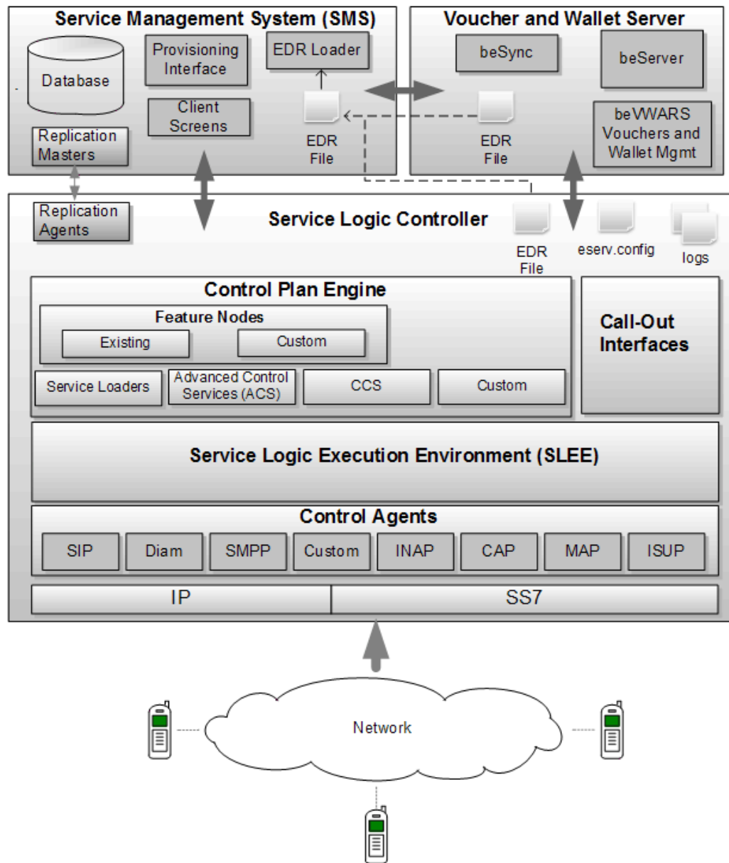
Figure 1-1 Convergent Charging Controller System Elements
