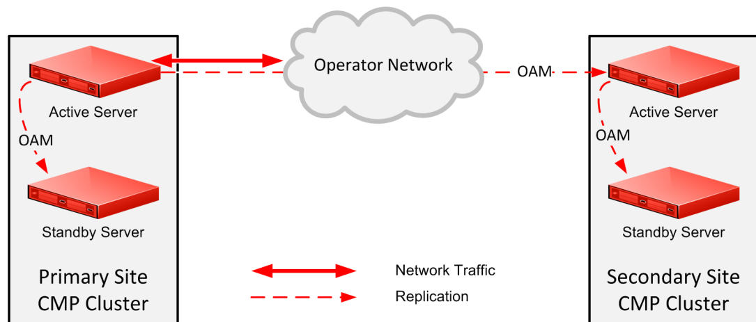
Figure 2-3 CMP Georedundancy
