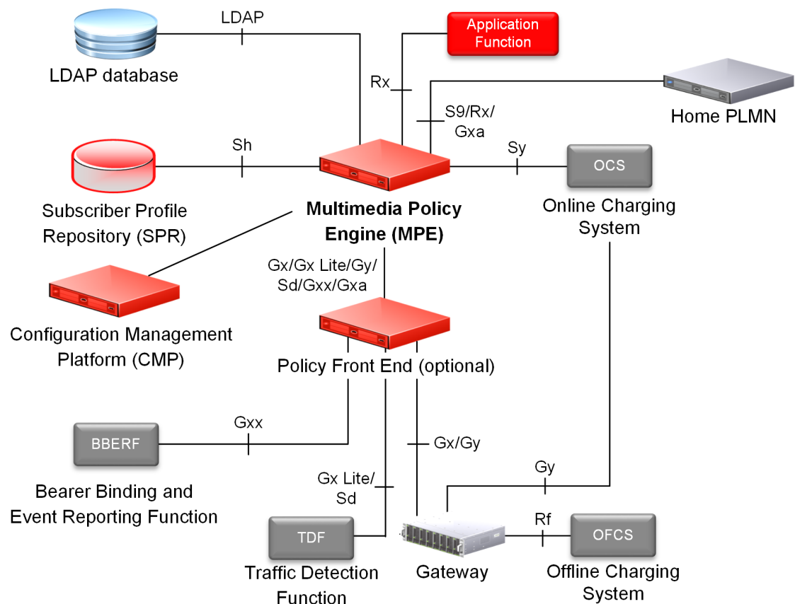
Figure 1-2 Diameter Interfaces to the Device
