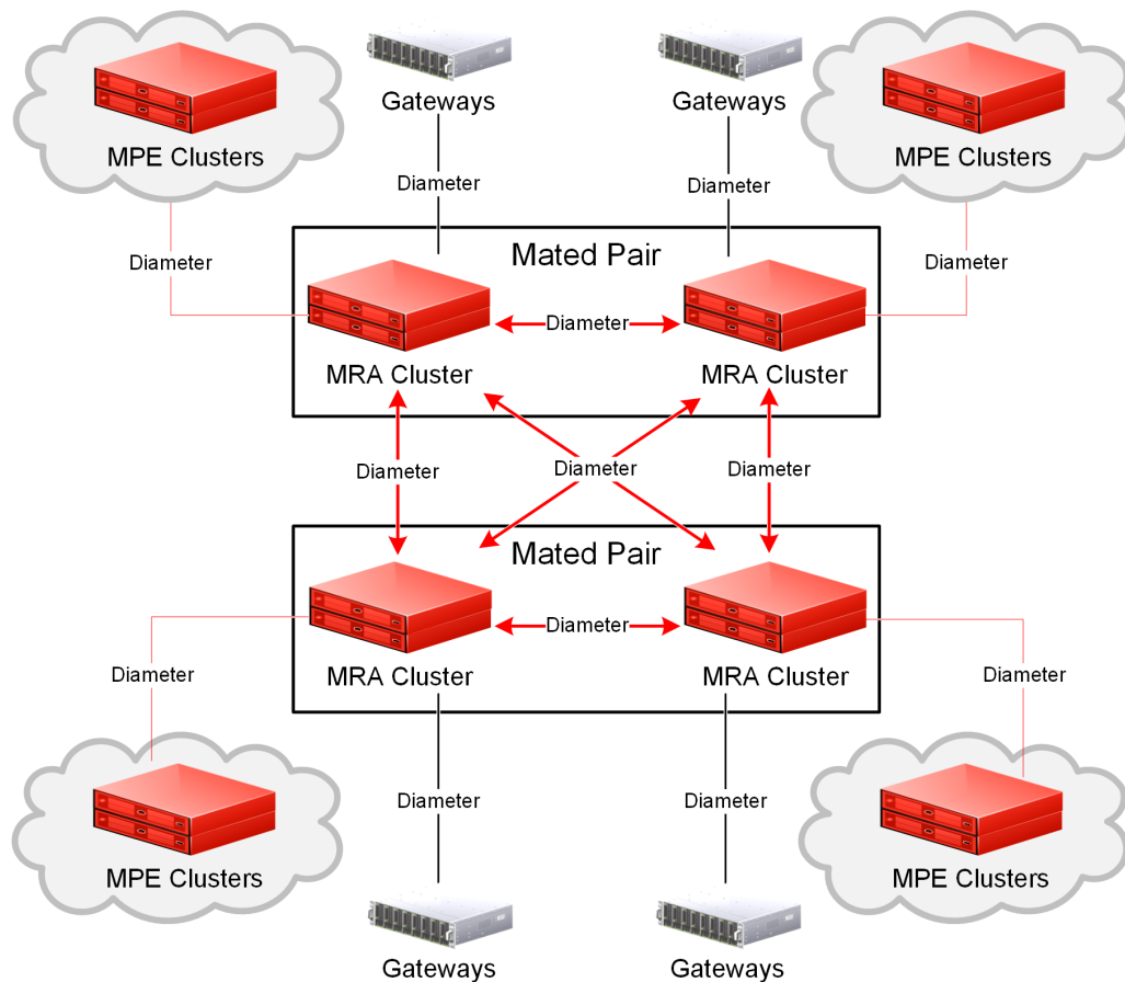
Figure 1-3 Typical MRA Network
