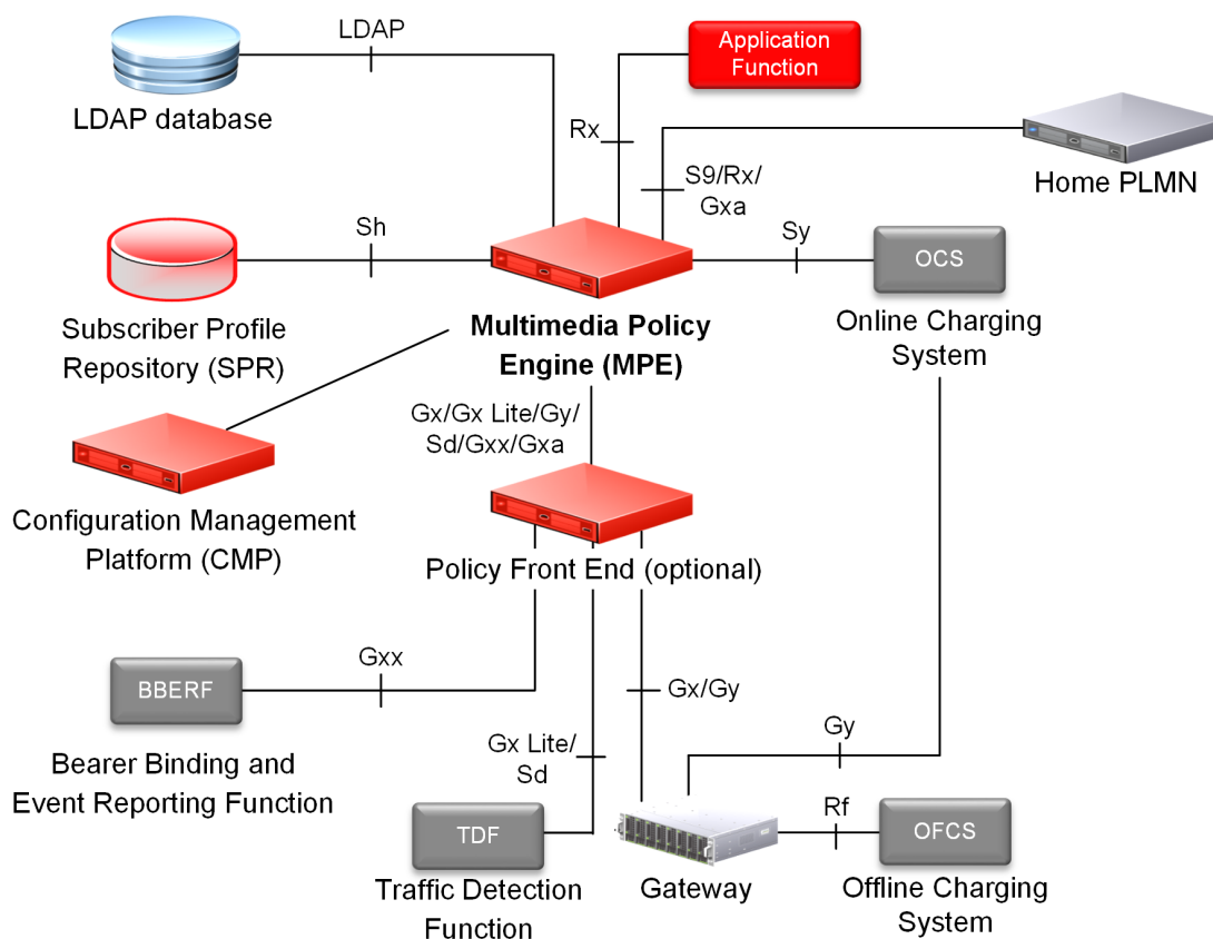
Figure 1-2 Diameter Interfaces to the MPE Device
