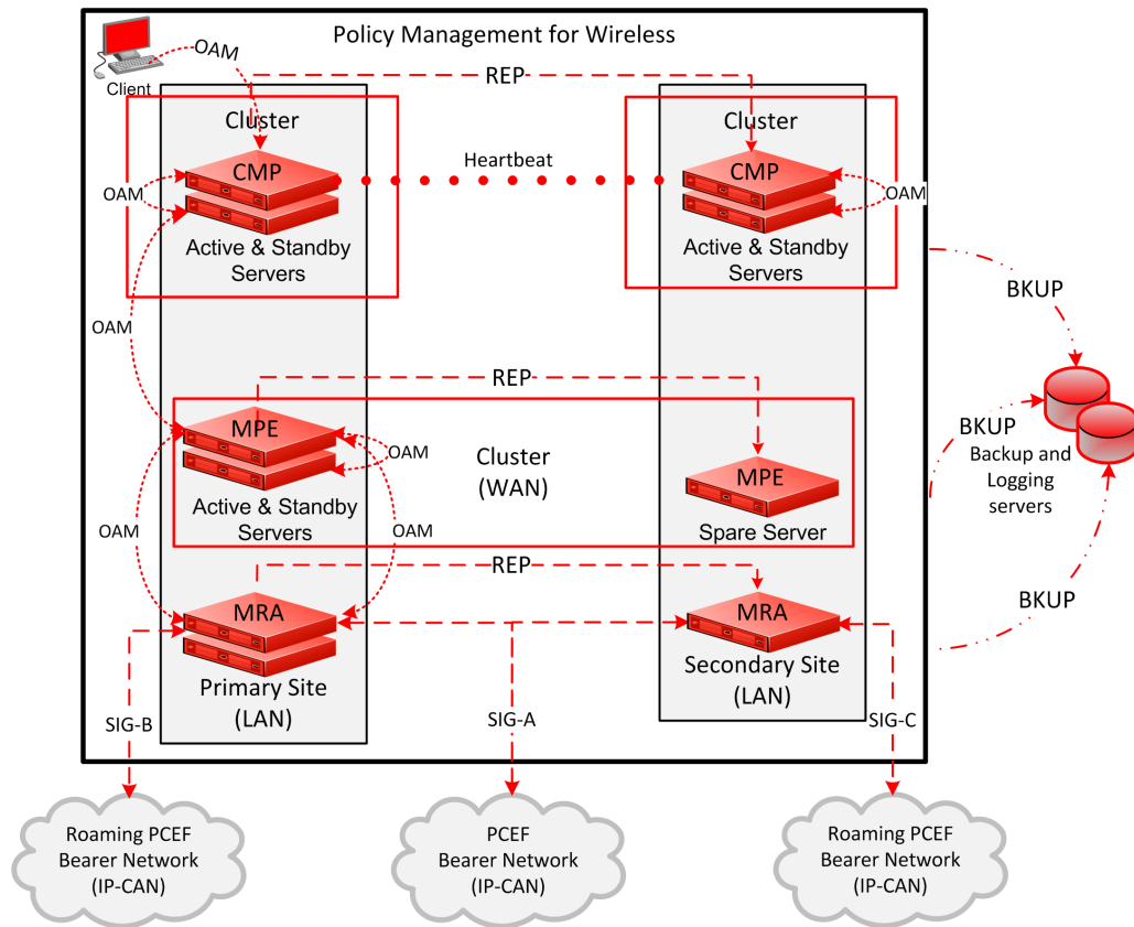
Figure 2-5 Wireless Georedundant System with Spare CMP Cluster
