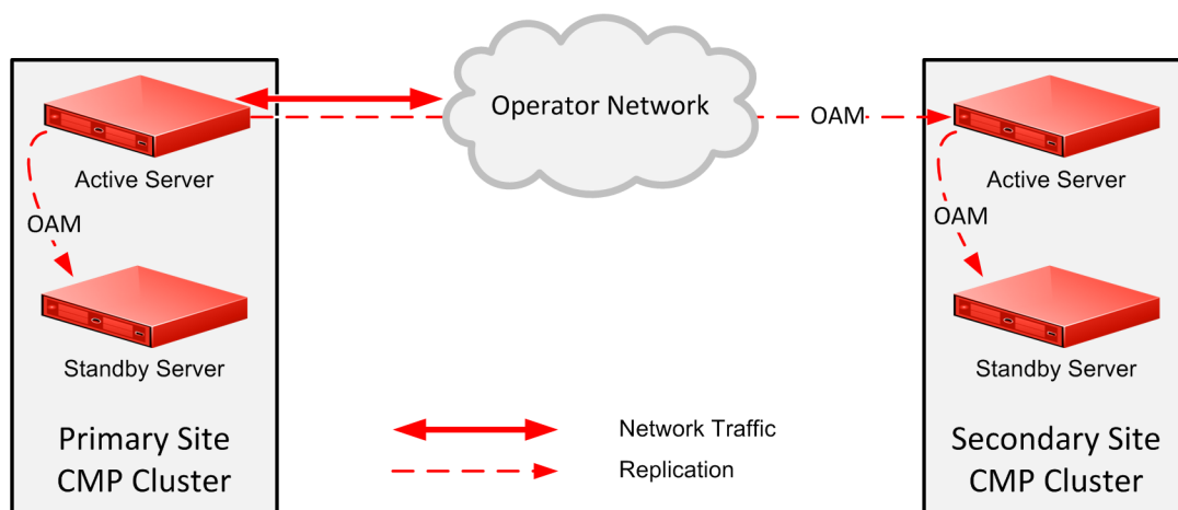
Figure 2-3 CMP Georedundancy
